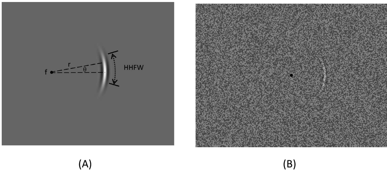
Figure 1. (A). The targets were Gabor arcs, centered at the fixation point, f , of different lengths defined in polar coordinates with radius r and angle \theta . For a better comparison with the literature, we reported the target size in HHFW, or half-height full width. (B) The target embedded in a binary noise mask.
