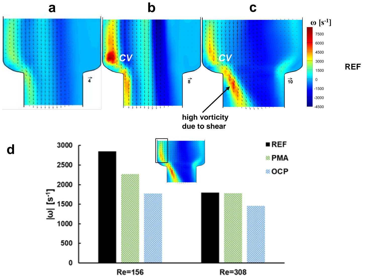
Fig. 13. Time-averaged velocity vectors over vorticity contour plots illustrating the recirculation pattern at the geometrical constriction of the valve-replica for the reference liquid: (a) Re=76 , (b) Re=156 and (c) Re=308 . The experimental uncertainty U_{\bar{\omega}} lies in the range 0.6-1.0%. (d) Comparison of spatially-averaged planar vorticity values at the constriction location for the three liquids examined. The vorticity values are averaged in the window shown in the inset of the figure, while the uncertainty associated with the spatially averaged values is of the order of 4%, slightly higher compared to the respective for the bend layout due to the reduced dimensions of the sampling window and, thus, number of averaging points.
