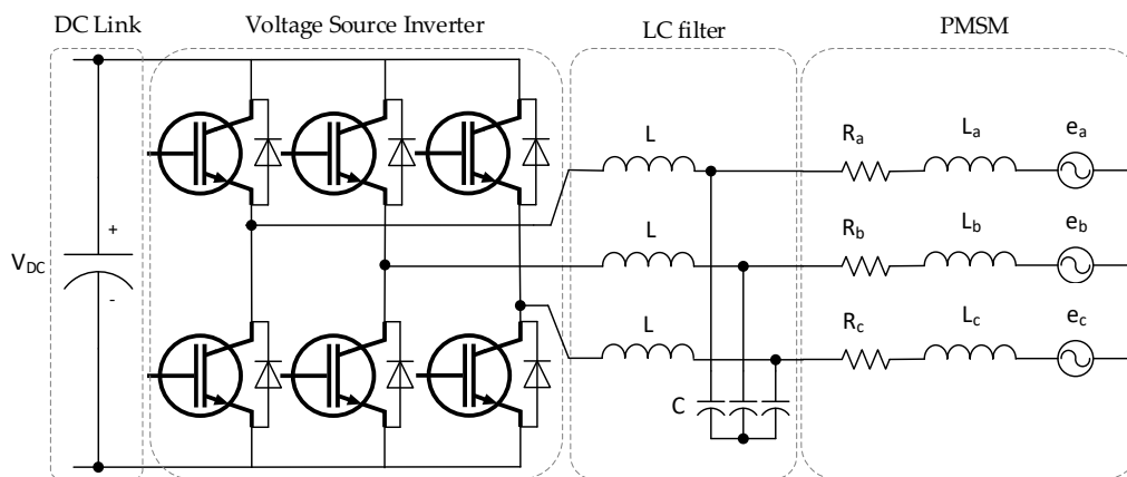
Figure 5.5. Circuit diagram of VSI and PMSM [142]
