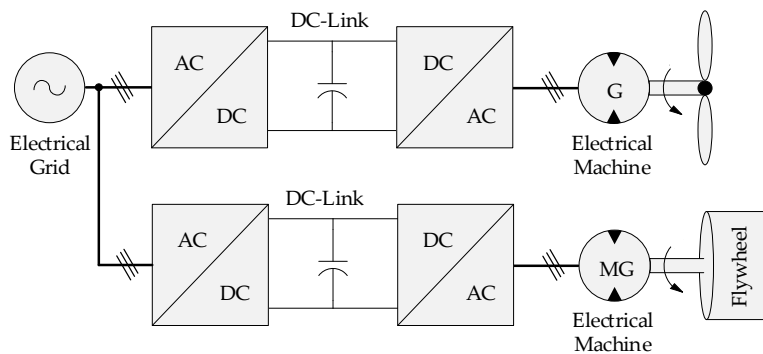
Figure 2.5. FESS with a BTB converter directly connected to the grid
