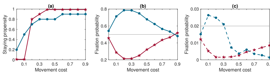
Figure 8. Complete graph, population size 50. Cooperators dominate defectors in a mixed population for all movement costs but the highest one. (a) Equilibrium staying propensities in a mixed population; (b) the fixation probabilities of cooperators and defectors with equilibrium staying propensities in a mixed population; (c) the fixation probabilities of mutant cooperators and mutant defectors in a resident defector and cooperator population, respectively, where both cooperators and defectors inherit equilibrium staying propensities from the mixed population. Legend: defectors—red with star markers for data points, cooperators—blue with round markers for data points; mixed population—solid line, mutants—dashed line; neutral drift fixation probability—solid grey line.
