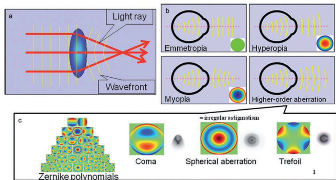
Figure 1.4. The differences in the concepts of a lens or an optical system in geometrical and physical optics (a). Effect of refractive errors on the wavefront (b). The wavefront of the perfect eye, that is an emmetropic eye without any aberrations, is shown as a perfect plane that is perpendicular to the line of sight. The wavefront in a myopic eye has a bowl-like (concave) shape with the peripheral wavefront more advanced than the central wavefront. The wavefront of the hyperopic eye has a hill-shape (convex shape) with the central wavefront more advanced than the peripheral wavefront. The wavefront of an eye with irregular astigmatism has an irregular and complex shape. The first to sixth orders Zernike
