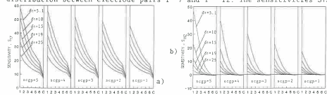
Fig. 8. Variations of sensitivities a) S_{17} and b) S_{12} with region position (radial regions); \delta_1 and s_{cgp} in mm
