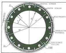
Fig. 1. Cross section of a 12-electrode capacitance system for flow imaging (not in scale)
