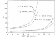
Fig. 4. Variation of K_c with electrode angle, \theta
