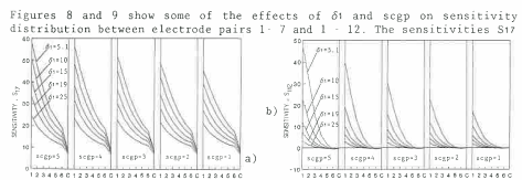
Fig. 8. Variations of sensitivities a) S_{17} and b) S_{12} with region position (radial regions); \delta_1 and s_{cgp} in mm
