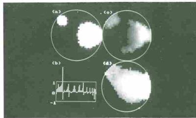
Fig.5. (a) Same flow phase distribution model as that shown in Fig.4a; (b) capacitance data \lambda_{ij} of flow model (a), calculated for a sensor with R_2 - R_1 = 20\text{mm} and with other sensor parameters being the same as those stated in Fig.4b; (c) same as in Fig.4c; (d) same as in Fig.4d.
