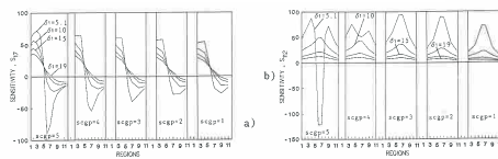
Fig. 9. Variations of sensitivities a) S17 and b) S12 with region position (regions on arc); \delta and scgp in mm
