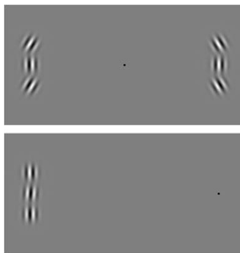
Fig. 1. Demonstrating repulsion and assimilation. The visual system exaggerates the orientation contrast between the (45°) tilted flankers and the vertical elements in the top panel. Small orientation differences, on the other hand, are effectively squelched. Thus, vertical flankers in the bottom panel can cause the small (4°) tilt to go unnoticed
