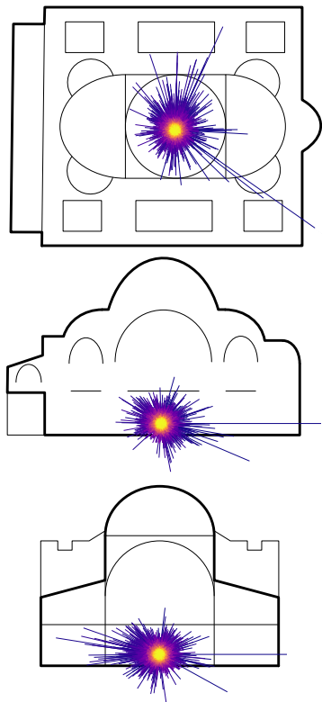
Fig. 3. Plan and elevation direction of arrivals.
