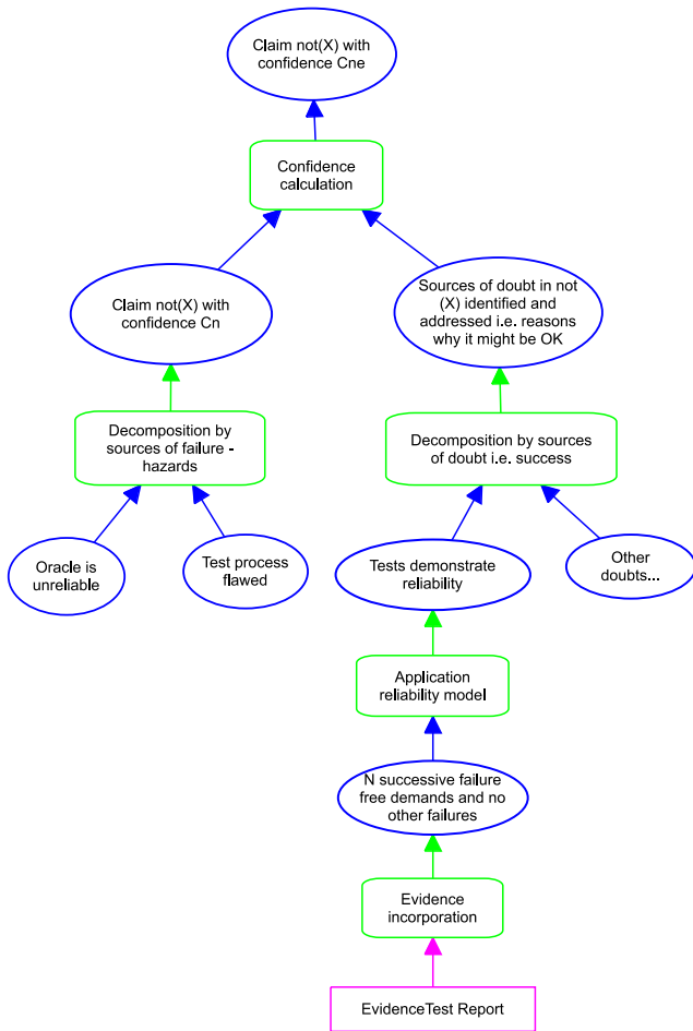
Figure 9. Systematically Derived Countercase
