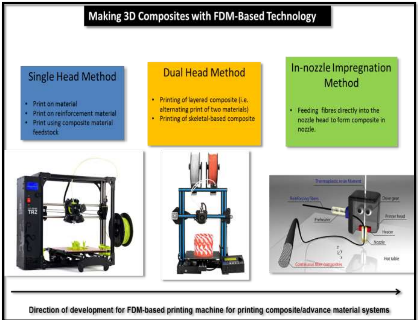
Figure 9 Development of FDM for advanced fabrication capabilities [5]
