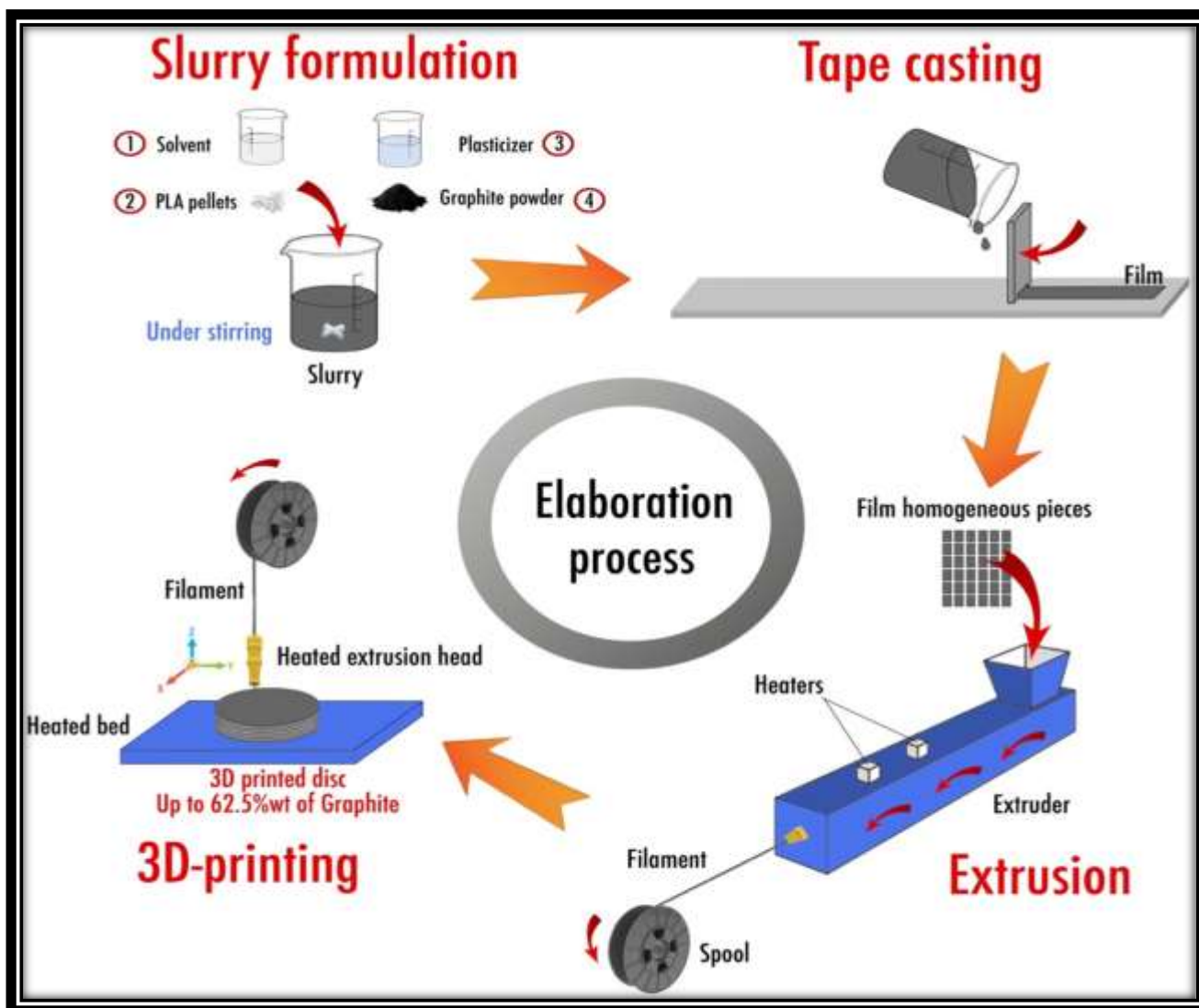
Figure 16 Elaboration process of the 3DP fabrication of graphite/PLA composite disc for Lithium-ion batteries. Adapted with permission from [96]. Copyright 2018, American Chemistry Society.
