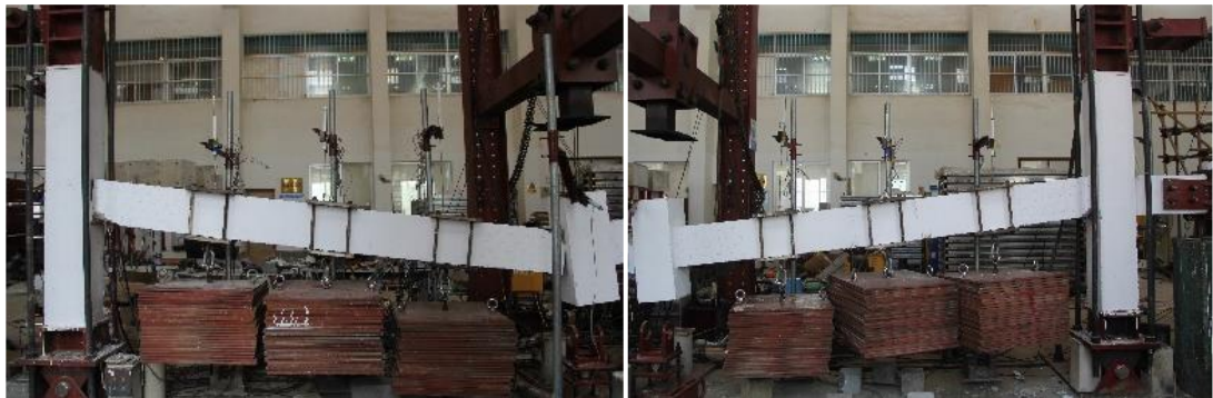
Figure 5 Crack pattern and local damage of UPPC-DL (from the author)
