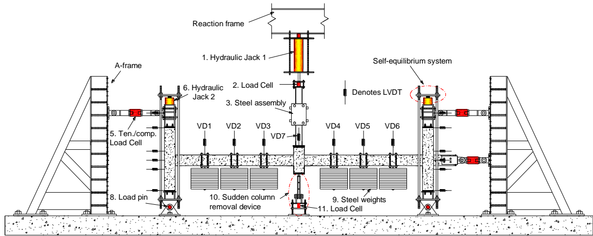
Figure 2. Test setup
