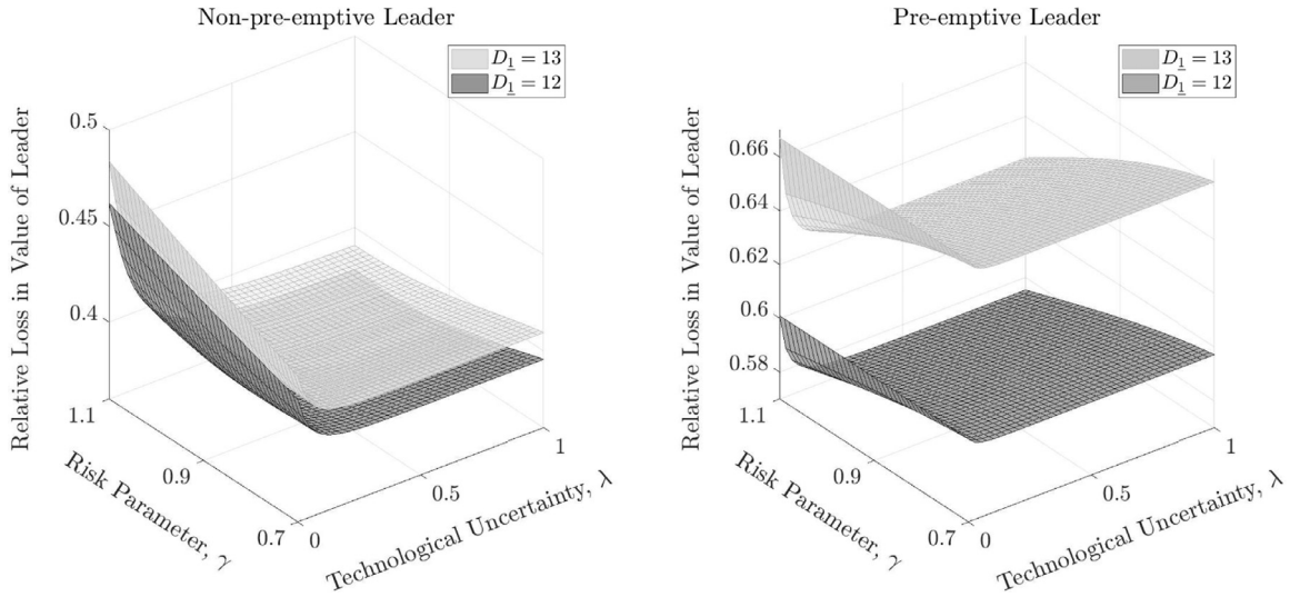
Fig. 11. Relative loss in the value of the non-pre-emptive (left panel) and pre-emptive leader (right panel) versus \gamma and \lambda for D_2 = 21 .
