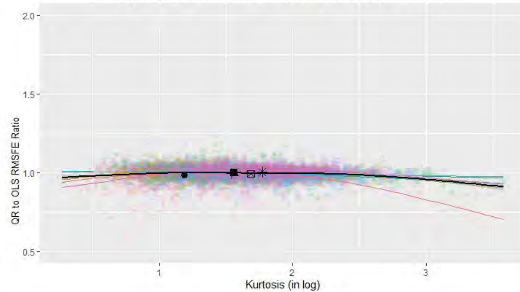
Figure 3b. Tail-Heaviness Effect on FIR of OLS under RMSFE
