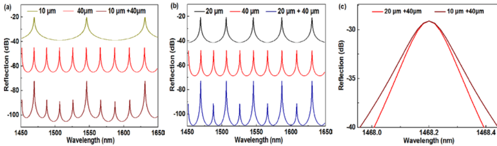
Fig. 3. (a) Simulated output spectrum of single set of cascaded FP cavities ( L = 10\ \mu\text{m} or 40\ \mu\text{m} ) and two sets of parallel structured cascaded FP cavities. (b) Simulated output spectrum of single set of cascaded FP cavities ( L = 20\ \mu\text{m} or 40\ \mu\text{m} ) and two parallel structured cascaded FP cavities. (c) Comparison of the spectral peaks for the parallel structured cascaded FP cavities with different separations.
