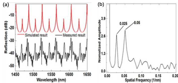
Fig. 4. The experimental and simulated output spectra of the device sample with (a) L_1 = 20\ \mu\text{m} , L_2 = 40\ \mu\text{m} ; frequency spectrum of the device sample with (b) L_1 = 20\ \mu\text{m} , L_2 = 40\ \mu\text{m} .
