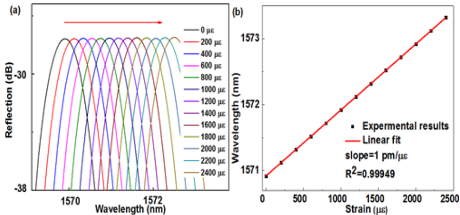
Fig. 6. Response of the device to strain. (a) Reflection spectra at different strains; (b) The peak wavelength shift versus strain.
