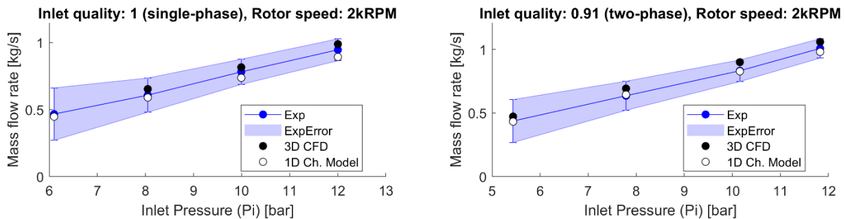
Figure 7: Expander mass flow rate for different inlet pressures at single and two-phase conditions, \epsilon_v = 2.4 , clearance (interlobe, radial, HP and LP End face): 100 \times 100 \times 50 \times 200 \mu\text{m} , 2000RPM
