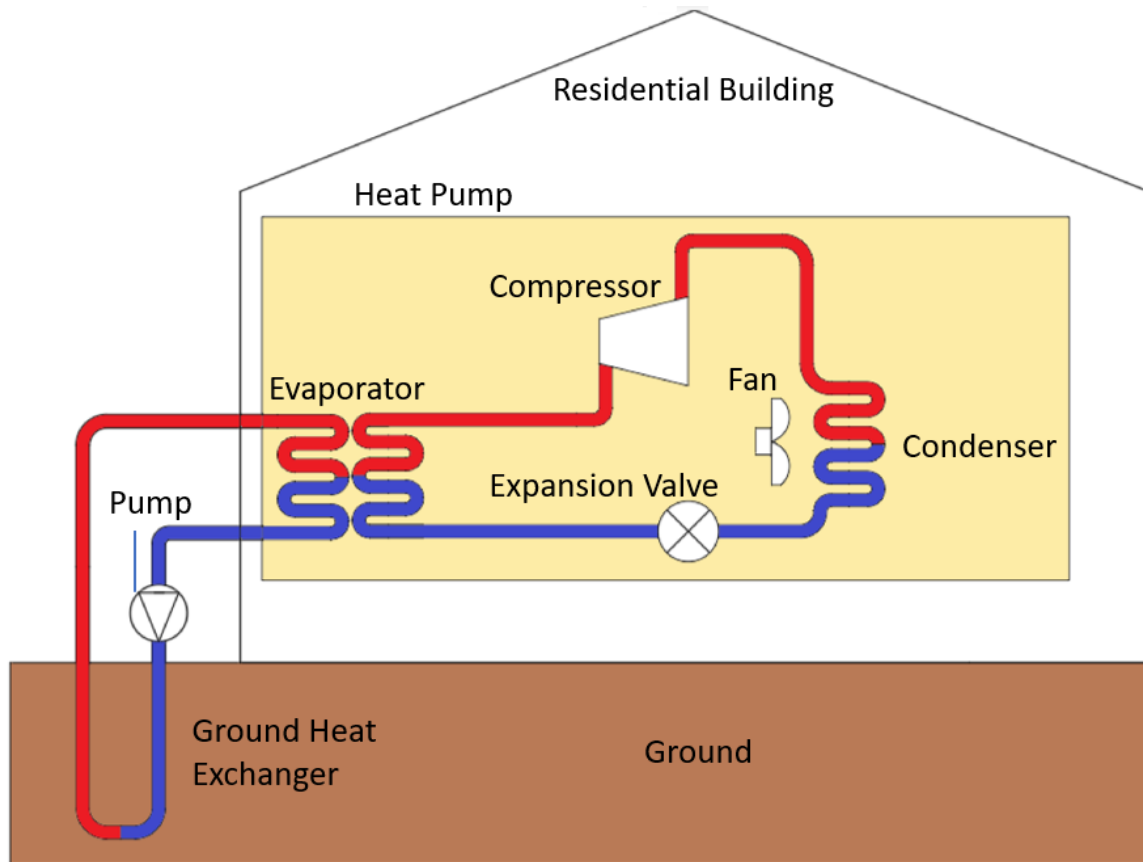
Figure 6: Ground source heat pump in heating mode
