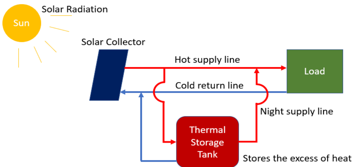
Figure 5: Solar heating system coupled with a thermal storage tank
