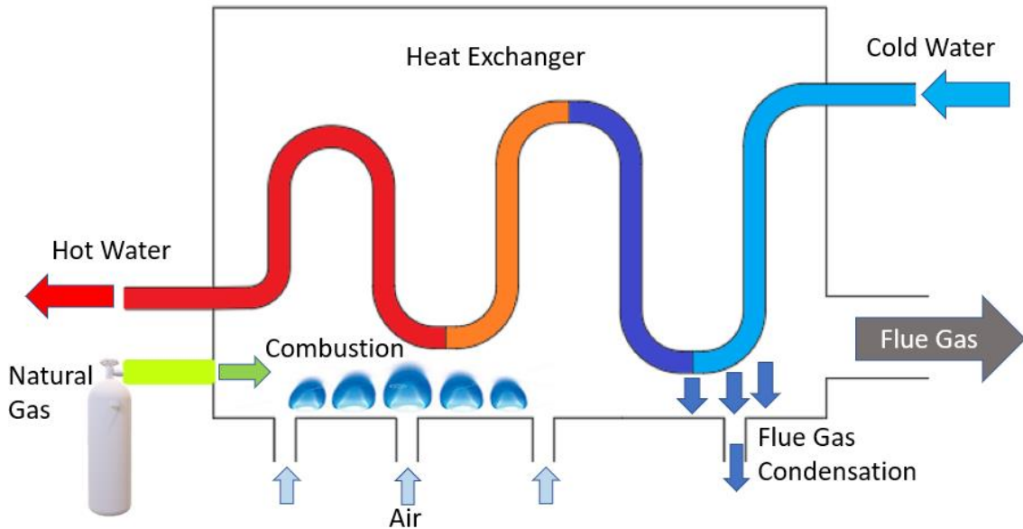
Figure 3: Natural gas condensing boiler
