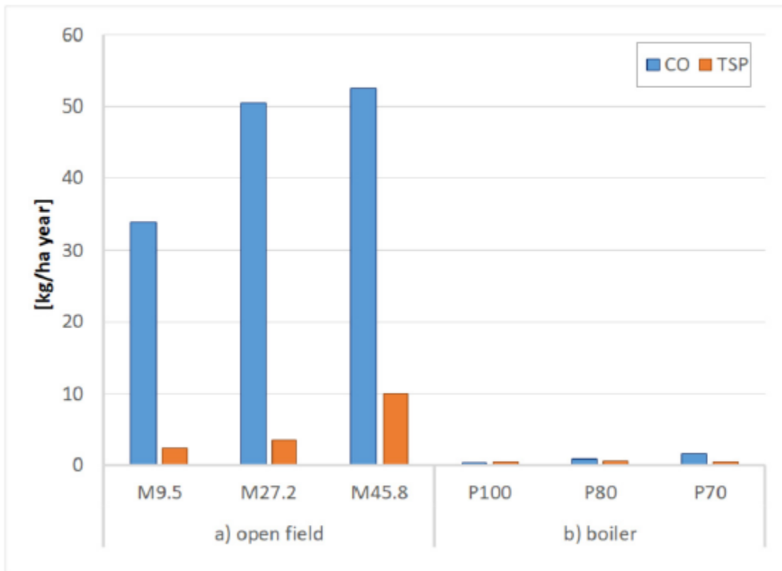
Figure 2: Yearly emissions due to burning pruning vine residues in open field and pellet boilers [67]
