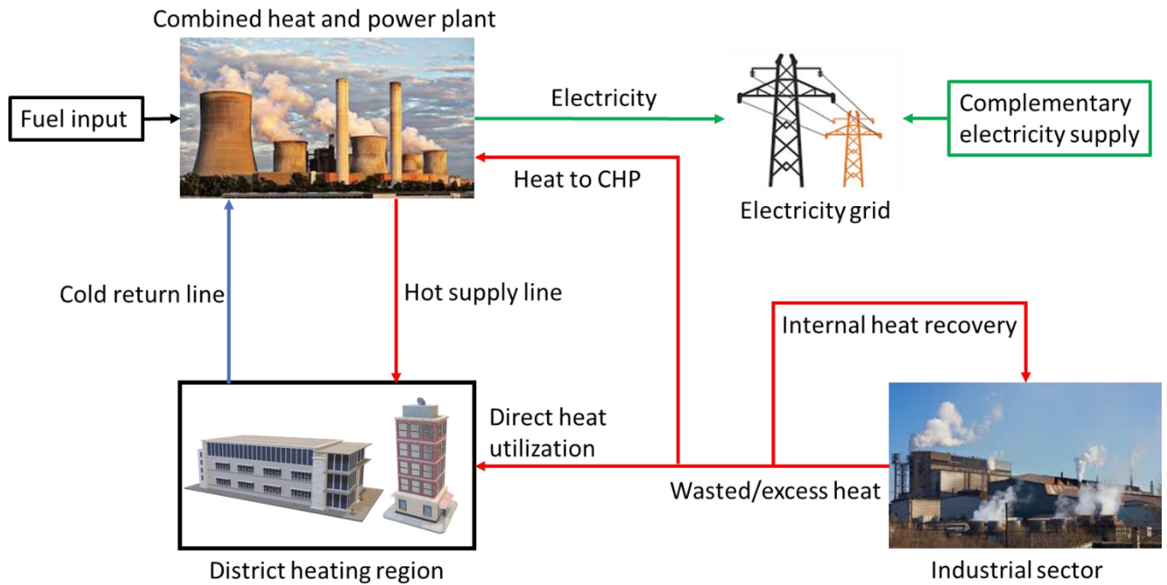
Figure 8: District heating system supported with excess industrial heat
