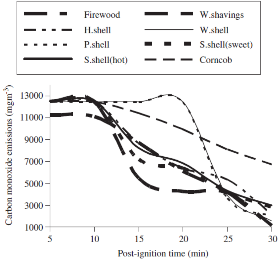
Figure 1: Carbon monoxide emissions of selected biomass fuels with respect to the time after ignition [62]
