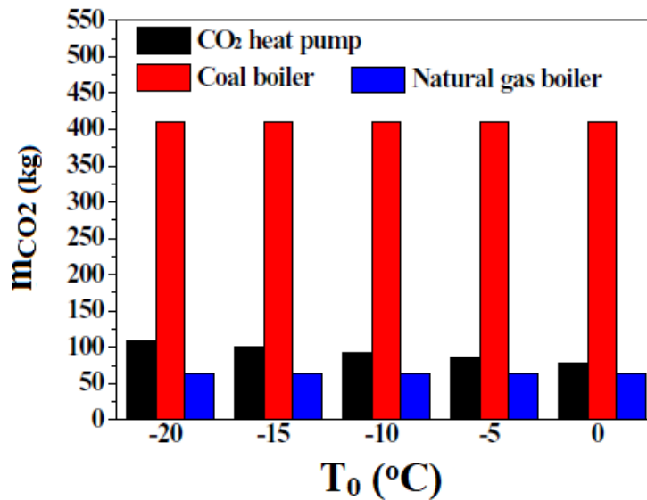
Figure 4: Comparison between coal, natural gas, and CO 2 heat pump [73]
