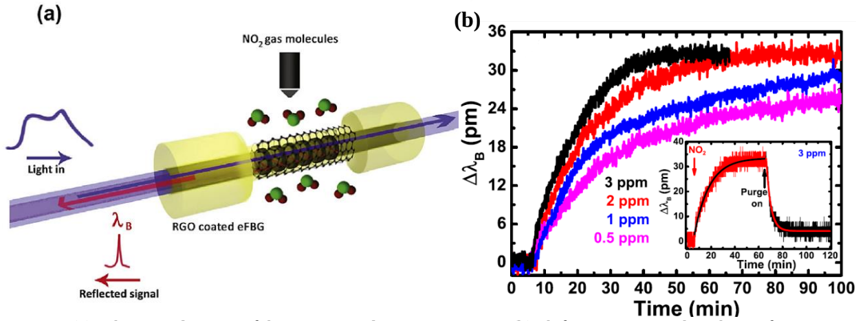
Fig 3. 29 (a) Schematic diagram of the rGO coated eFBG gas sensor (b) Shift in Bragg wavelength as a function of time for different concentrations of \text{NO}_2 gas. The inset shows one complete adsorption and desorption cycle for 3 ppm \text{NO}_2 gas exposure [84].
