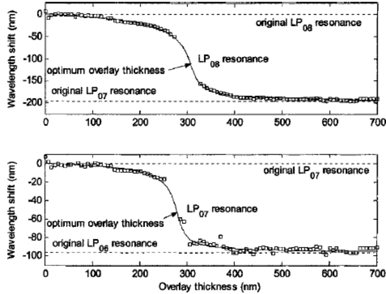
Fig 2. 19 Shift in resonance wavelength caused by coupling between the core mode and the seventh (LP 07 ) and the eighth (LP 08 ) cladding modes of the structure as a function of the thickness of the overlay. Open square, experimental values; solid curves, theoretical values [57].
