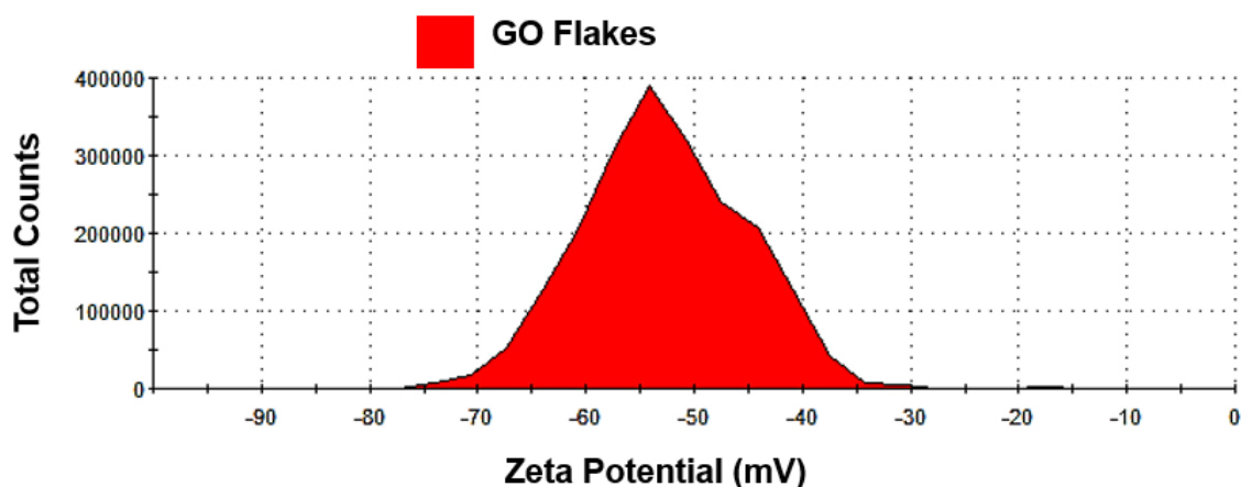
Fig 4. 11 Surface Zeta potential of GO flakes synthesised.
