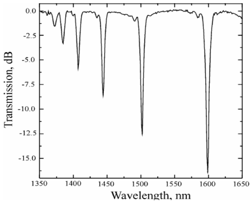
Fig 2. 7 Typical transmission spectrum of a LPG [3].
