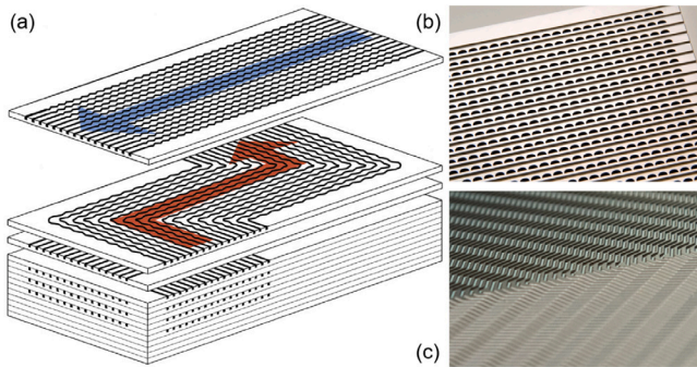
Fig. 8. (a) Typical PCHE: (b) flow paths and details of the diffusion-bonded core (c) and of an etched plate (courtesy of Heatric Meggitt UK).
