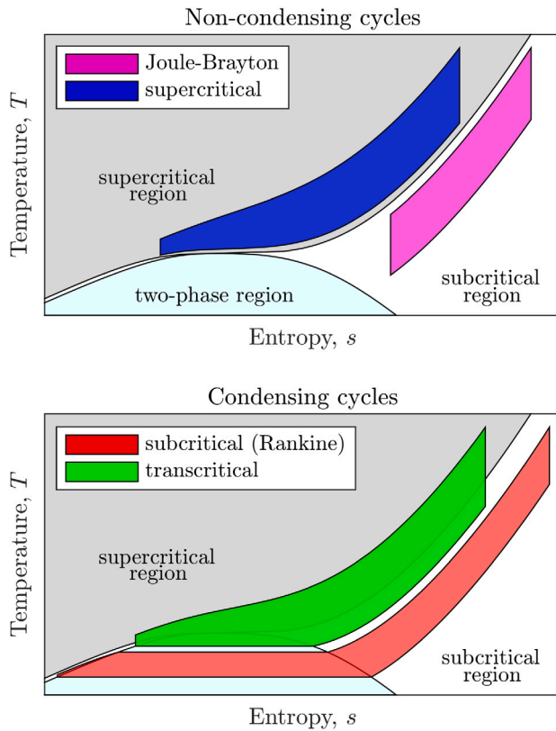
Fig. 3. Classification of thermodynamic power cycles. (For interpretation of the references to colour in this figure legend, the reader is referred to the web version of this article.)
