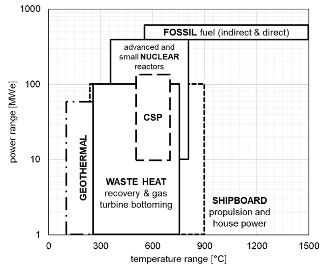
Fig. 12. Overview of s\text{CO}_2 power applications. Source: Elaboration from [217].
