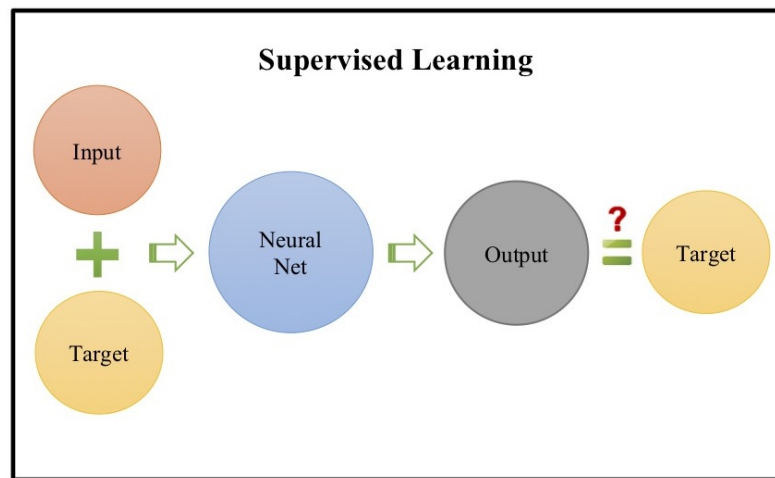
Fig. 2.6 Supervised Learning
