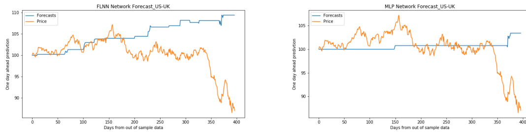
Fig. 10.6 US-UK data (orange) and trading simulation (blue) for the FLNN model (left) and the MLP model (right).
