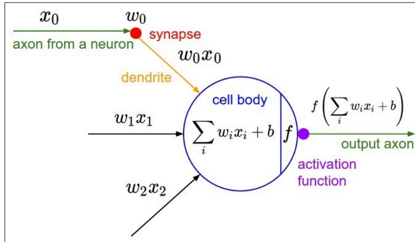
Fig. 2.2 The neuron model (Perceptron)
