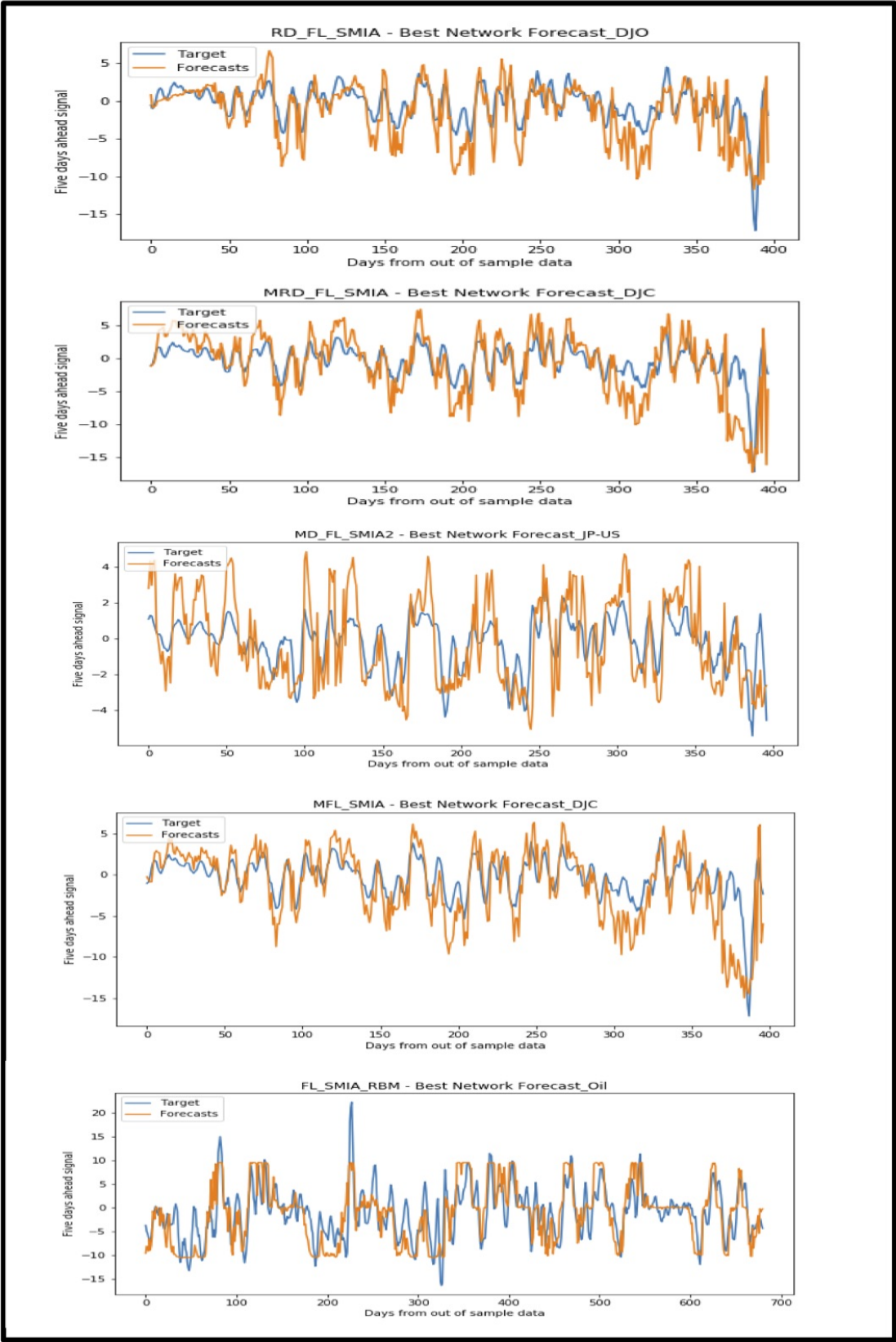
Appendix 1-2: The best forecasting on testing data for five days ahead prediction
