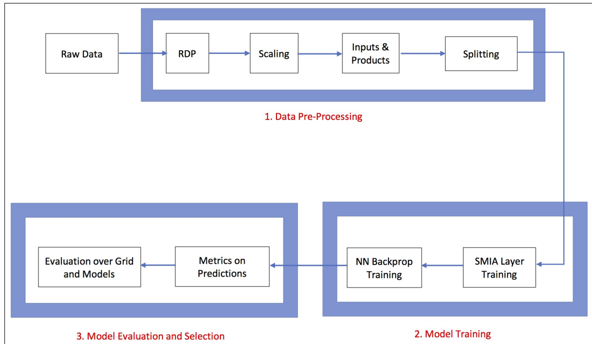
Fig. 3.1 The processing pipeline used in this study.
