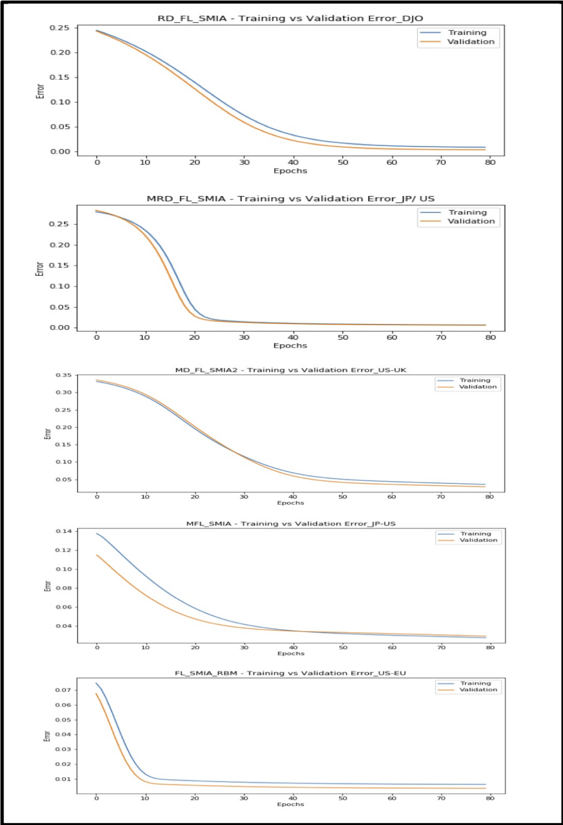
Appendix 2-2: The best MSE results for training and validation errors for five days ahead prediction
