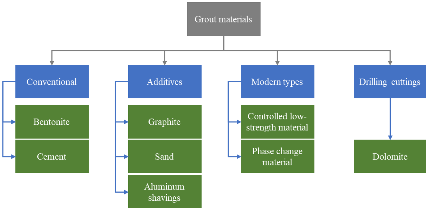
Figure 3: Commonly used grout materials in geothermal energy systems
