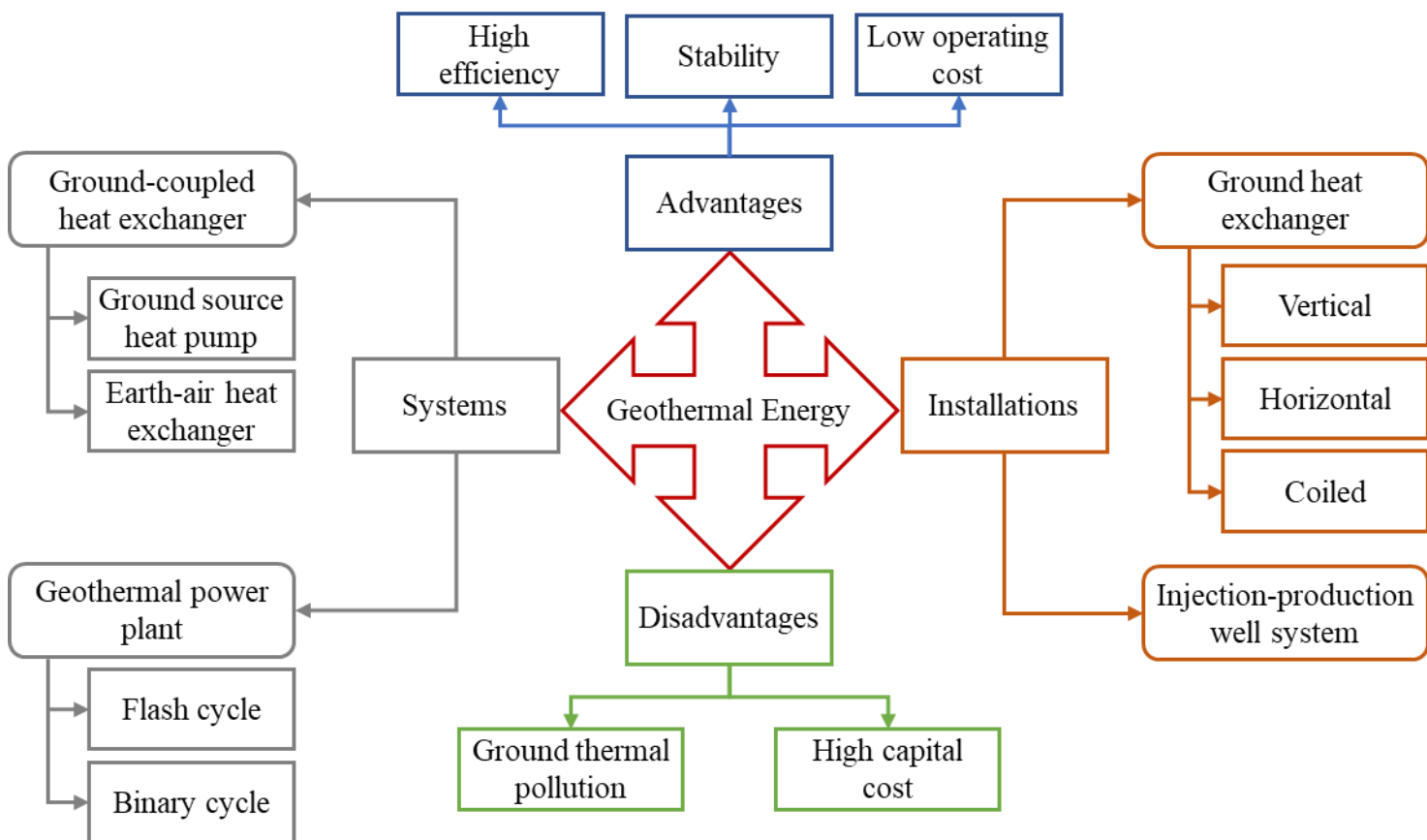
Figure 1: The utilizations and characteristics of geothermal energy systems
