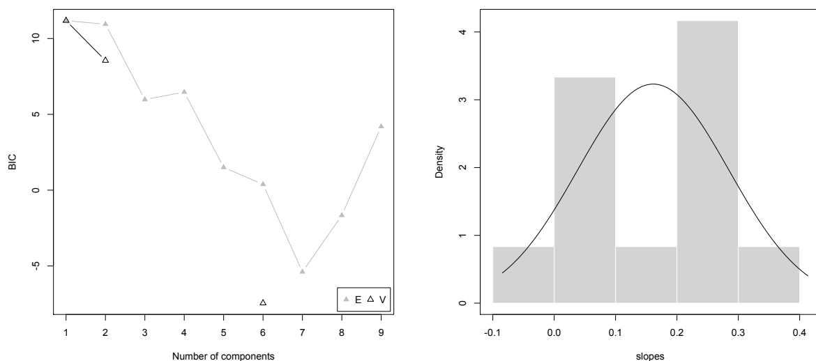
Figure 34. The Bayesian Information Criterion (BIC) indicates that a single population best fits the histogram of the slopes in Fig.33 (left), with the resulting Gaussian distribution plotted on top of the histogram of the slopes from Fig.33 (right).
