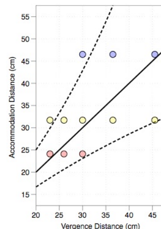
Figure 30. Vergence / Accommodation Conflict. Left: Graph from Hoffman et al. (2008) illustrating the ‘zone of clear single binocular vision’ ( \pm 1D ). © ARVO. Right: The various combinations of vergence and accommodation tested in Experiment 2 using trial lenses. ● = –
