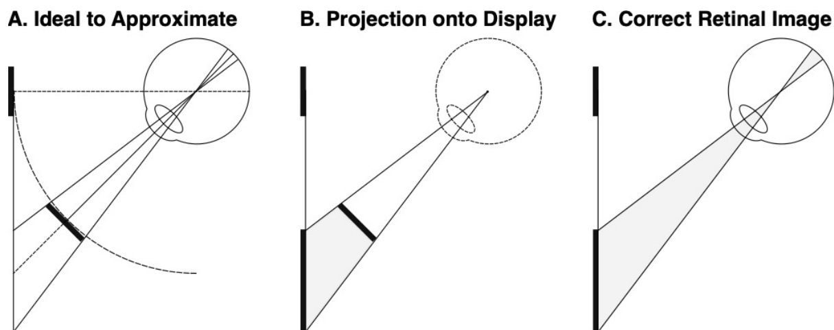
Figure 39. Illustration of the principle behind OpenGL projection in Experiment 3.
