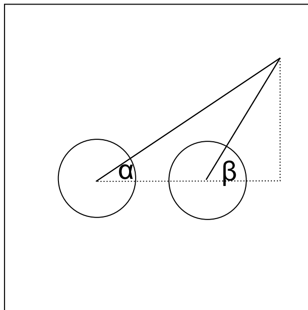
Figure 15. Vertical disparity is the difference between \alpha and \beta .
