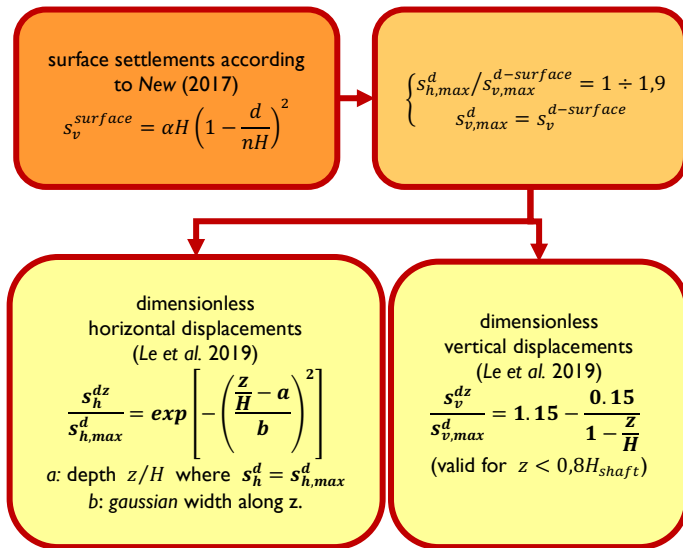
Figure 1. Prediction procedure proposed by Le et al. (2019).
