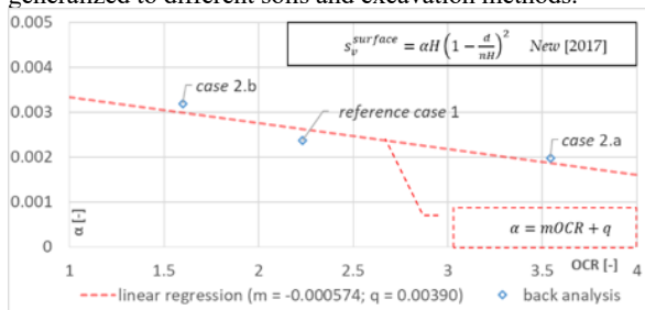
Figure 7. Coefficient \alpha in Eq. 1 as a function of OCR.
