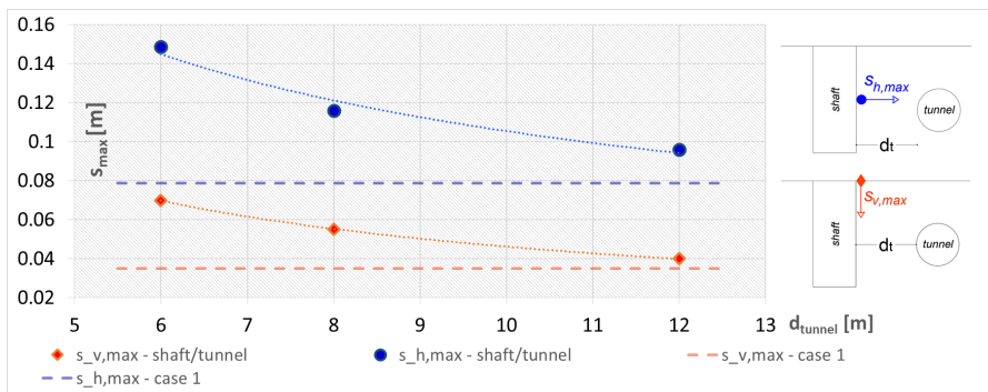
Figure 12. Influence of the net distance d_{\text{tunnel}} in the shaft/tunnel interaction problem.
