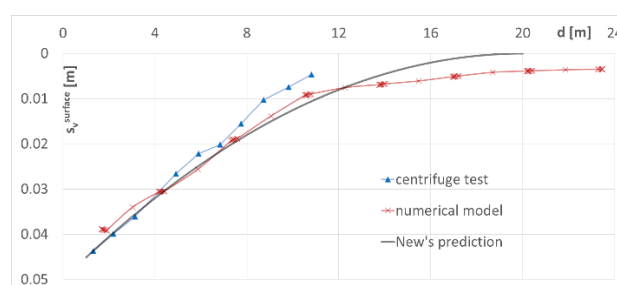
Figure 5. Computed settlement trough compared with centrifuge test results (Le et al., 2019) and New (2017) prediction (Eq.1, \alpha=0.0025 , n=1 ).
