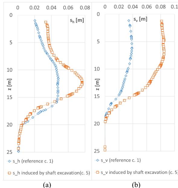
Figure 10. Interaction with an existing tunnel: horizontal (a) and vertical (b) displacements caused by the shaft excavation after tunnelling (case 5) compared to those of the reference case 1 ( d= 3m ).
