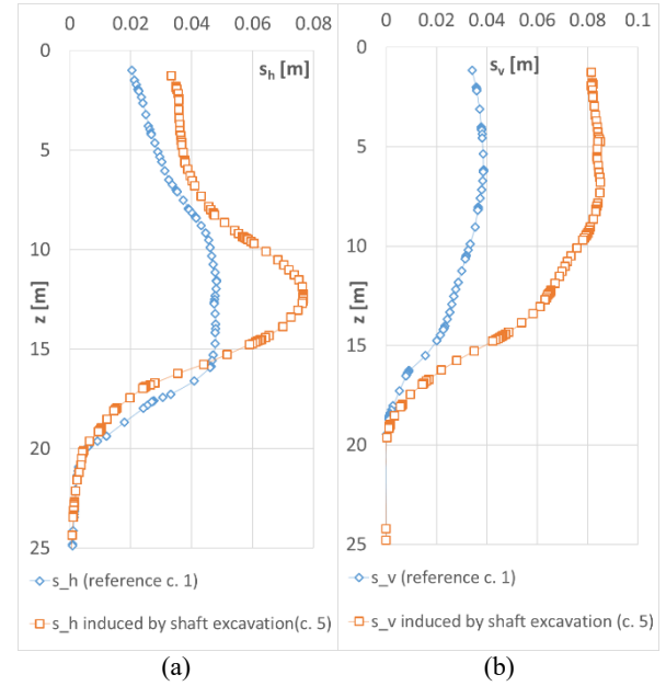
Figure 10. Interaction with an existing tunnel: horizontal (a) and vertical (b) displacements caused by the shaft excavation after tunnelling (case 5) compared to those of the reference case 1 ( d= 3\text{m} ).
