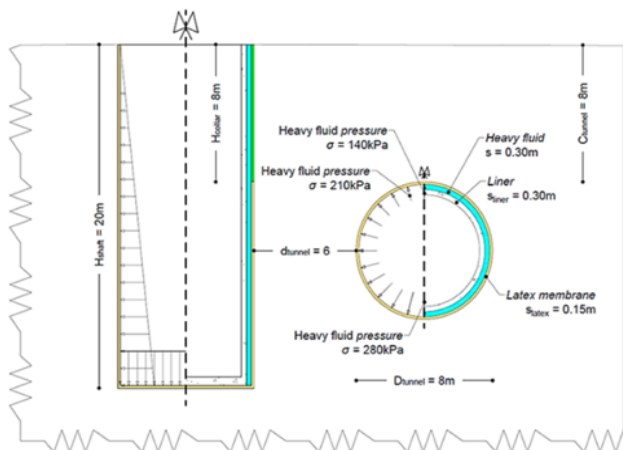
Figure 9. Geometry of the interaction problem shaft/tunnel (case 5).
