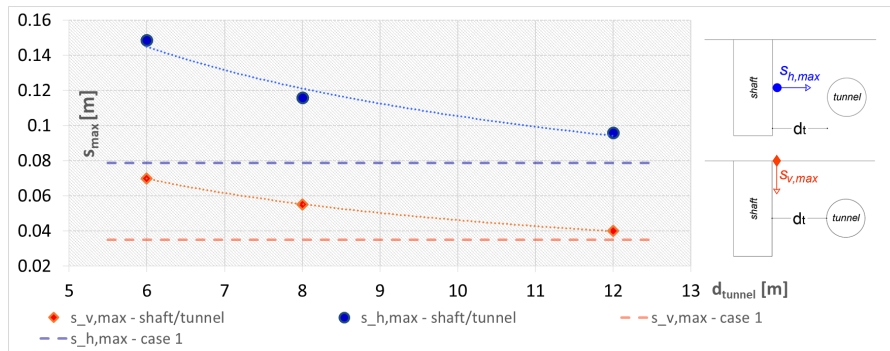
Figure 12. Influence of the net distance d_{\text{tunnel}} in the shaft/tunnel interaction problem.
