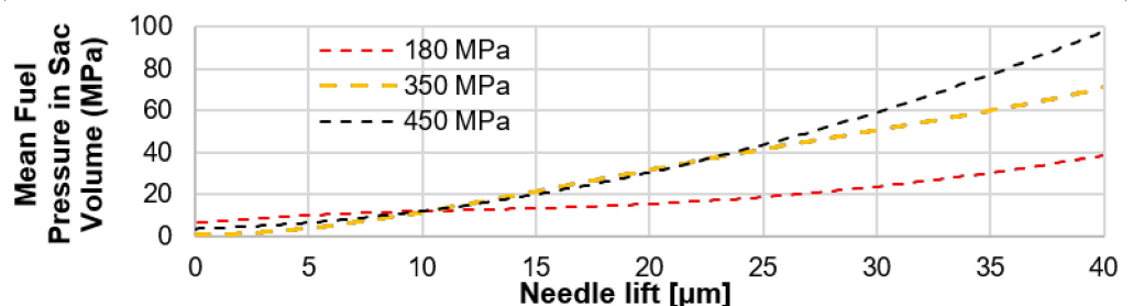
Figure 6. Temporal evolution of fuel pressure in the injector’s sac volume for lift increases from 2 μm to 40 μm during the plotted time.
