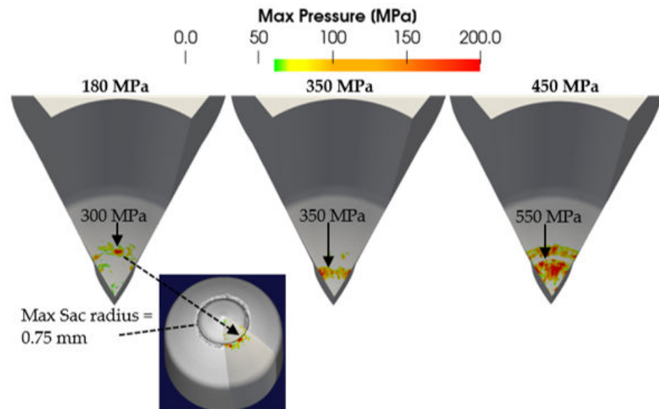
Figure 12. Spatial distribution of the accumulated pressure peaks on the surface of the needle valve. Strongest collapse events are located on the needle surface, reaching up to 550 MPa for the 450 MPa injection pressure case.
