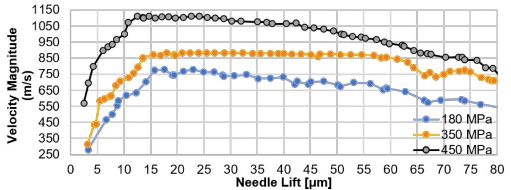
Figure 4. Temporal evolution of the maximum velocity magnitude at the narrowest point of the needle seat passage indicating the lift increase from 2 μm to 80 μm over the simulated time.
