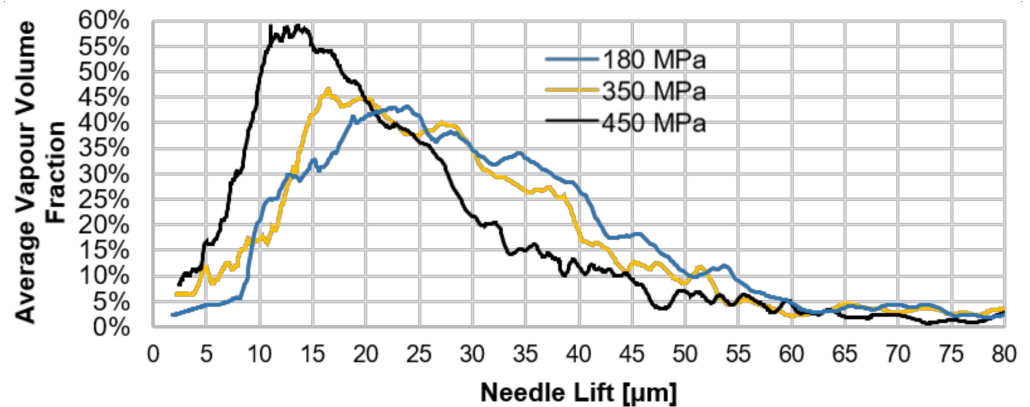
Figure 5. Vapor volume fraction in the injector volume during the early opening phase of the needle valve. The vapor volume is normalized by the sum of the needle seat passage volume below the narrowest point, the injector’s sac, and the orifice volumes. It is noted that at zero needle lift, the sac volume is 3.1 times larger than the volume of the orifice.
