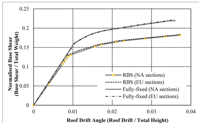
FIGURE 11 | NA vs EU sections normalized capacity curve comparison for 8-storey frame.
