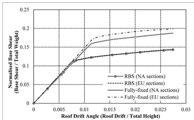
FIGURE 12 | NA vs EU sections normalized capacity curve comparison for 16-storey frame.
