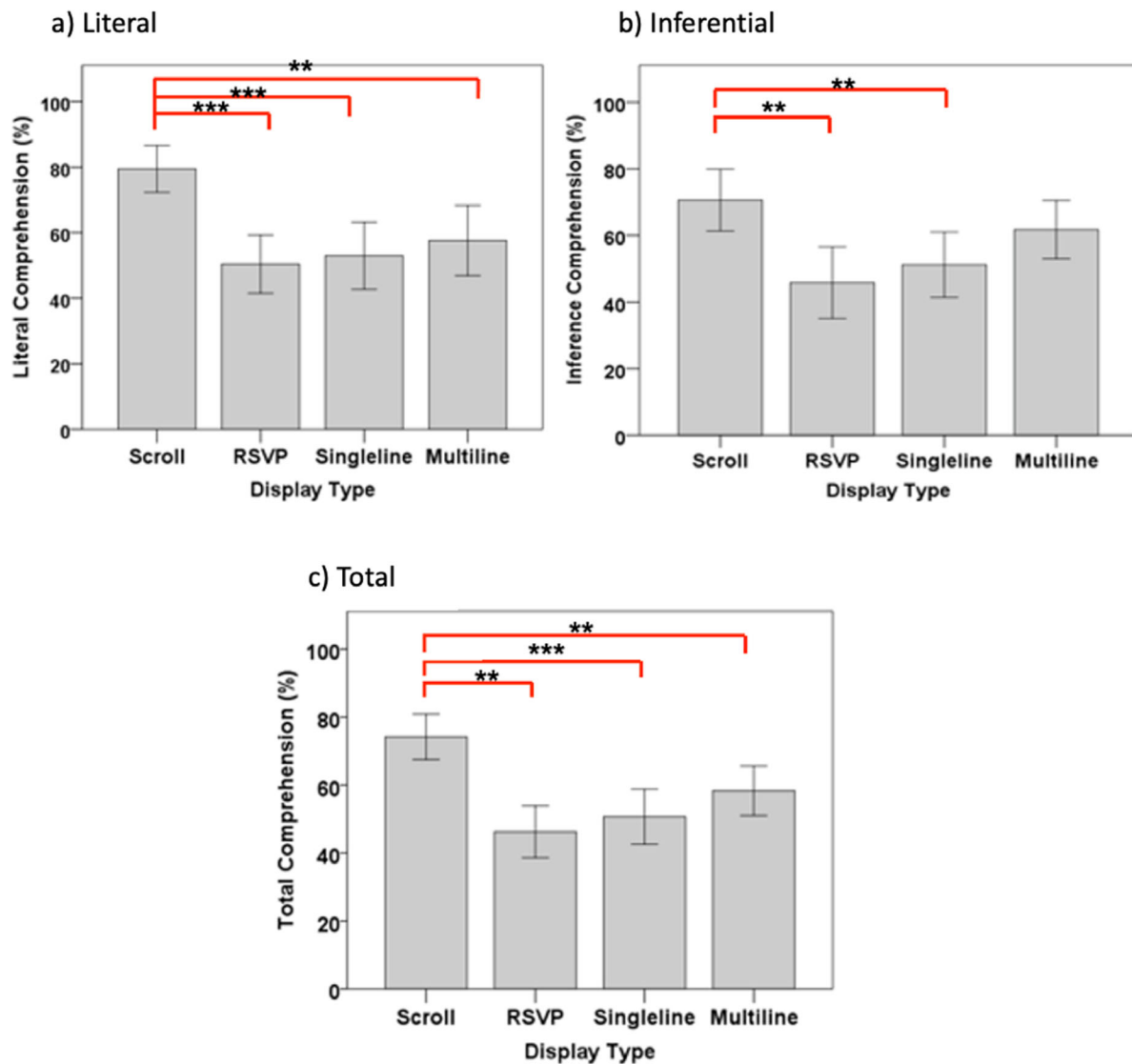
Figure 10. Average reading comprehension for macular degeneration participants across display formats: (a) literal comprehension, (b) inferential comprehension, and (c) total overall comprehension. *p < 0.05 ; **p < 0.01 ; ***p < 0.001 .
