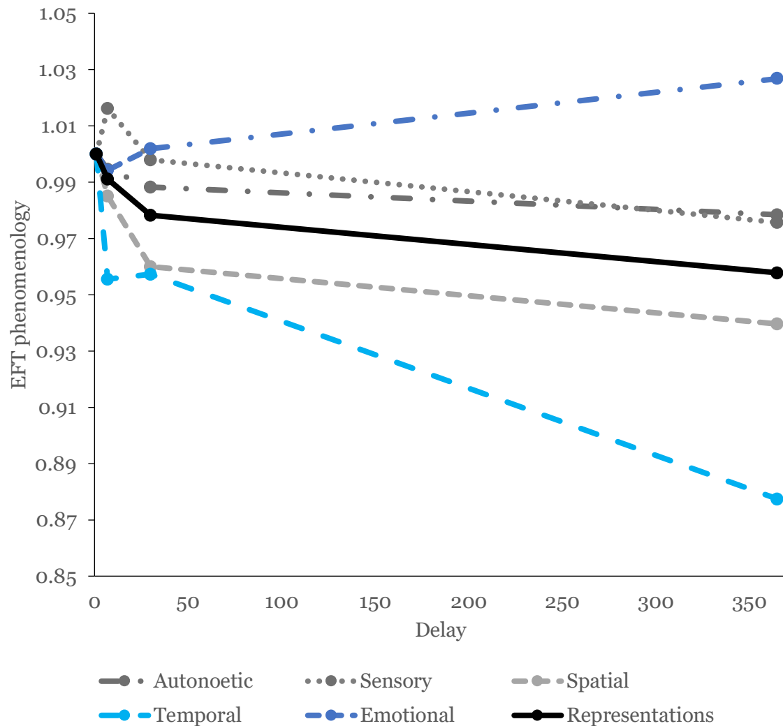
Figure 3.3: The representation richness variable and the 5 individual variables.
