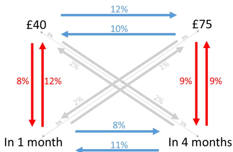
Figure 4.13: The means in table 4.19 that were greater than zero.
