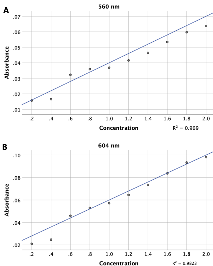
Figure 3. Linear regression analysis of absorption variations of different lithium concentrations in the region between 540-570 nm and 590-615 nm of the difference spectra. (A) Absorption variations at 560 nm representing the first peak. (B) Absorption variations at 604 nm representing the second peak. (P-value < 0.05)
