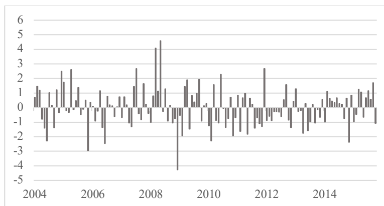
Figure 3.7. Residuals from linear regression of GBP/$ Currency and IMF EU Sugar Import Prices
