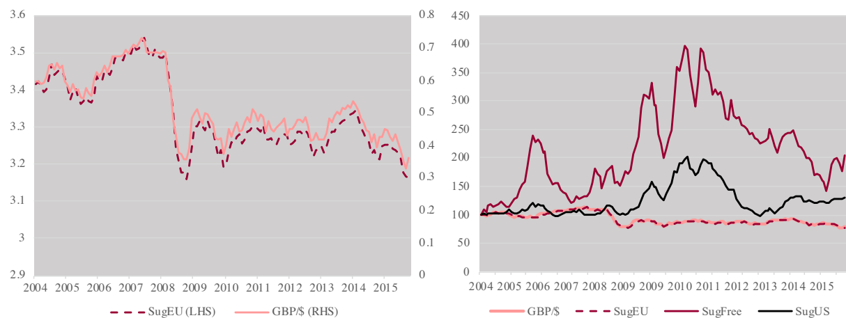
Figure 3.1. (Left) Natural Log of GBP/$ Exchange Rate and IMF EU Sugar Import Price Levels from 30th June 2004 to 31st March 2016, (Right) GBP/$ Exchange Rate and IMF Sugar (Free Market, US and EU) Price Levels Indexed to 100 at January 2004
