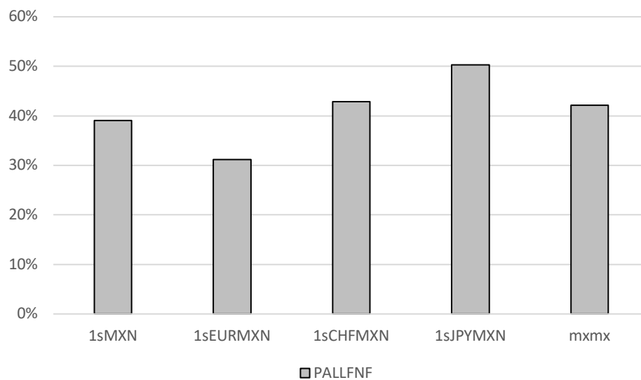
Figure 2.4. Mexico Currency Cross-Screening Correlations of All Commodity and Fuel (PALLNF) to Variable Base Currency Time Series and MSCI Mexico Equity Series (MX_E)
