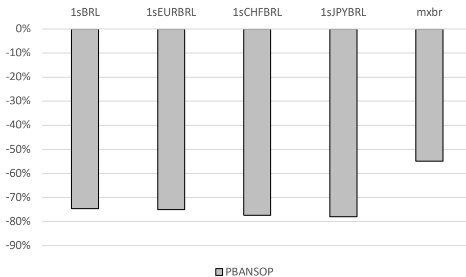
Figure 2.5. Brazil Currency Cross-Screening Correlations of Banana Commodity (PBANSOP) to Brazilian Real in Variable Base Currency Time Series' and MSCI Brazil Equity Series (BR_E)
