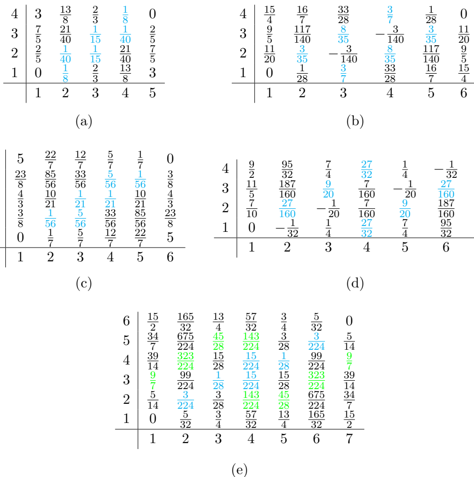
Figure 3. Here we list the first five possible examples of CBs that \Gamma(3) corresponds to: (a) p' = 6, p = 5 , (b) p' = 7, p = 5 , (c) p' = 7, p = 6 , (d) p' = 8, p = 5 , (e) p' = 8, p = 7 . Those appeared in the CBs are in cyan in the Kac tables. For (e), we also have another combination of CBs in green.
