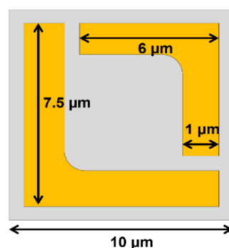
Figure 10. The schematic unit cell proposed from [204] to detect viruses. The periodic pattern is composed of the combination of large L and small L.
