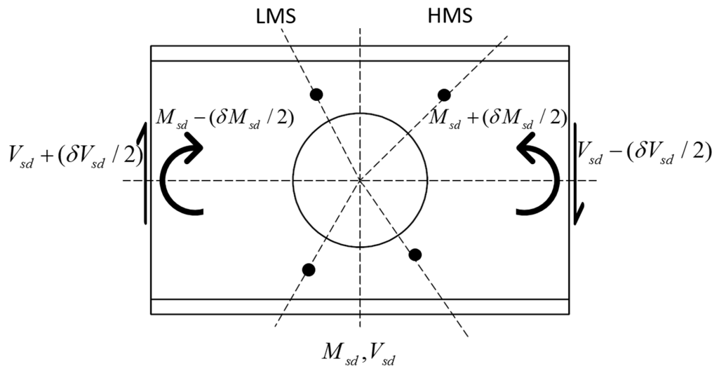
Figure 1: Vierendeel mechanism
