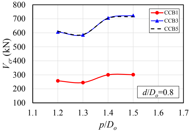
(a) d/D_o=0.8
