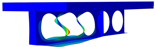
(c) CCB5: d/D_o=1.2 , p/D_o=1.2 and b_{we}/b_w=1.8
