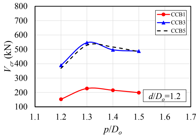
(e) d/D_o=1.2
