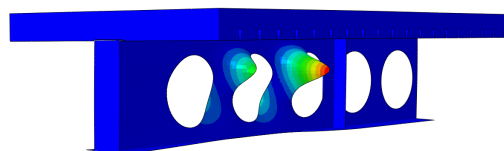
(f) CCB6: d/D_o=1.0 , p/D_o=1.3 , b_{wel}/b_w=3.8
