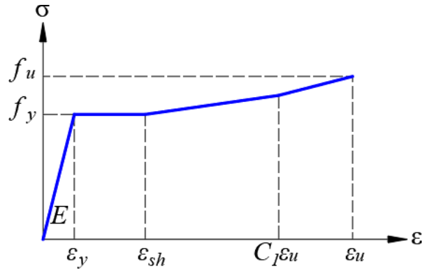
7 Fig. 2: Stress-strain relationship for steel [54]
