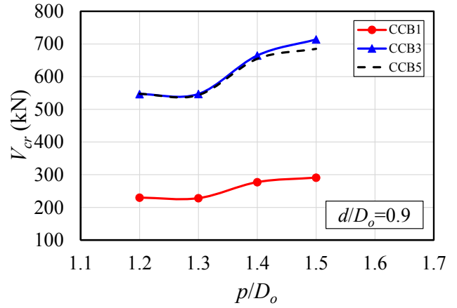
(b) d/D_o=0.9
