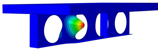
(b) CCB3: d/D_o=1.2 , p/D_o=1.5 and b_{we}/b_w=1.0
