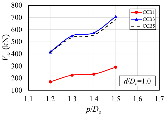
(c) d/D_o=1.0
