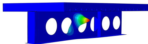
(b) CCB6: d/D_o=0.8 , p/D_o=0.8 , b_{wel}/b_w=2.9
