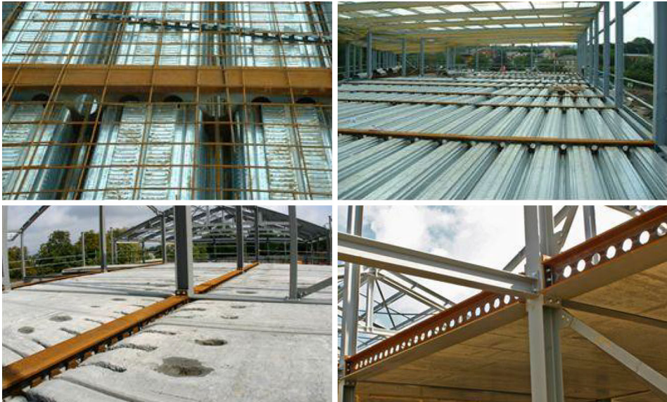
Figure 1. USFB used with profiled steel decking (top) and with pre-cast concrete unit (bottom) [13].
