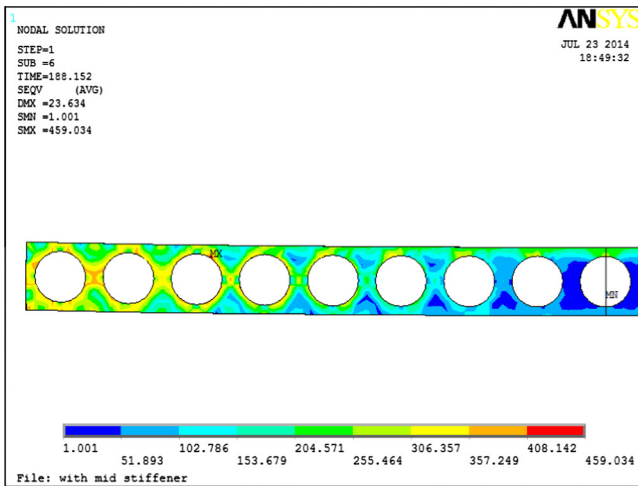
Fig. 8. Von Mises stress plots for cellular and topology optimised beams at yield load level.
