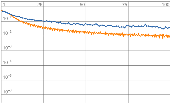
FIG. 6. Training loss (orange) and validation loss (blue) for the network (6.1) with l = 3 , n = 415 and (n_1, n_2, n_3) = (256, 64, 16) , learning the absence/presence of Higgs pairs for SLMs on the manifold #5032 with |\Gamma| = 4 . A feature-enhanced dataset (3.4) is used.
