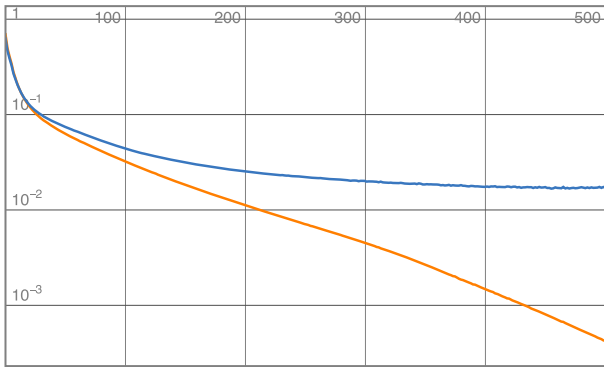
FIG. 3. Training loss (orange) and validation loss (blue) for the network (4.1) as a function of training rounds for the data from CICY #5302 and |\Gamma| = 4 with |K| \leq 5 .
