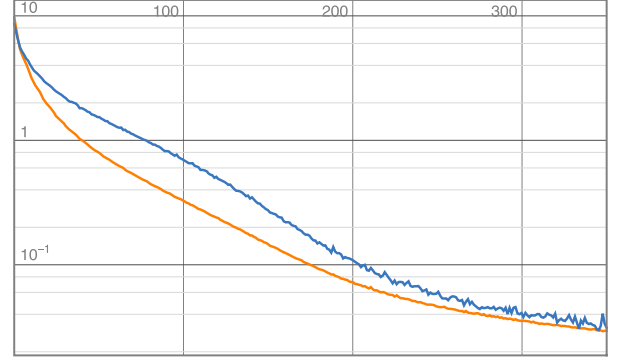
FIG. 7. Training loss (orange) and validation loss (blue) for the network (6.4) with l = 3 , n = 415 and (n_1, n_2, n_3) = (256, 64, 16) , learning the number of Higgs pairs for SLMs on the manifold #5032 with |\Gamma| = 4 . A feature-enhanced dataset (3.4) is used.
