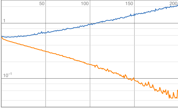
FIG. 5. Training loss (orange) and validation loss (blue) for the network (6.1) with l = 4 , n = 30 and (n_1, n_2, n_3, n_4) = (256, 128, 64, 16) , attempting to learn the absence/presence of Higgs pairs for SLMs on the manifold #5032 with |\Gamma| = 4 . The increase of the validation loss indicates a failure to generalize.
