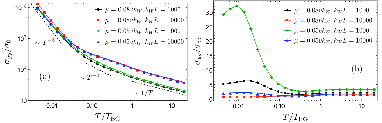
Figure 6. Temperature dependence of \sigma_{yy} and \sigma_{zz} as in Fig. 5 but for fixed boundary angle \alpha = 0 and with \mu/vk_W \in (0.05, 0.08) and k_W L \in (1000, 10000) . Panel (a) shows \sigma_{yy}/\sigma_0 vs T/T_{BG} on double-logarithmic scales. Panel (b) shows \sigma_{yy}/\sigma_{zz} vs T/T_{BG} for the same parameters on a semi-logarithmic scale.
