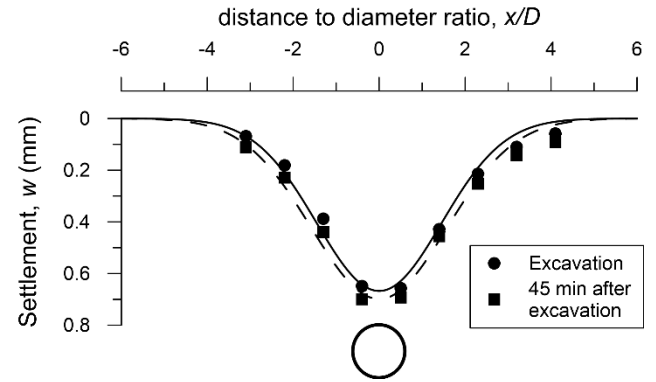
Fig. 4. Surface settlements obtained from centrifuge test.
