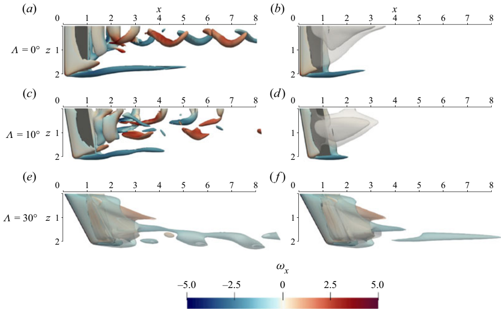
Figure 7. Same as figure 6 but for sAR = 2 at \alpha = 22^\circ . For clarity additional contour of Q = 0.1 transparent is included for \Lambda = 30^\circ .
