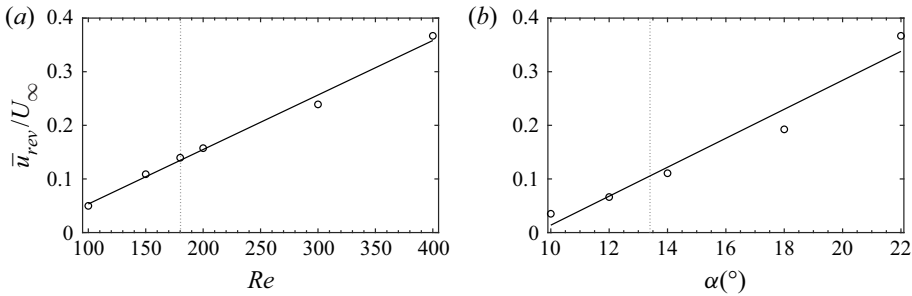
Figure 16. Dependence of the maximum reverse streamwise velocity component on (a) Re at (sAR, \Lambda, \alpha) = (4, 0^{\circ}, 22^{\circ}) and (b) on \alpha at (sAR, \Lambda, Re) = (4, 0^{\circ}, 400) . Lines correspond to a least-squares fit of the data points.
