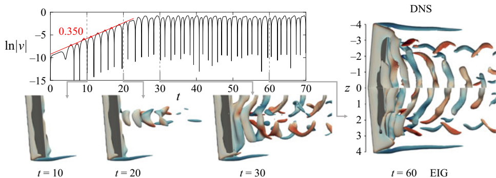
Figure 17. Growth of the global mode for (sAR, \Lambda, \alpha, Re) = (4, 5^\circ, 22^\circ, 400) showing the time history at point P(x, y, z) = (4, 0, 2) and flow field evolution at selected times. On the right, the resulting flow field is also compared with the DNS result.
