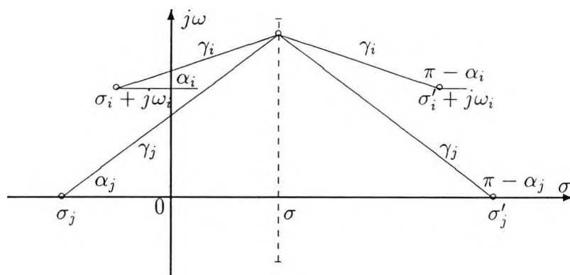
Figure 5.8: Root distribution of the sum of two n -th order polynomials
