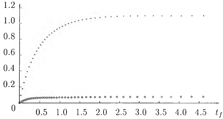
Figure 3.1: Singular Values of the Output Controllability Grammian of Example 3.1
