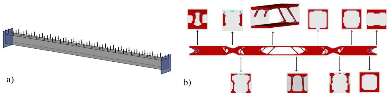
Figure 5. 3D optimisation input (a) and resulting topology with cross-sectional slices (b)
