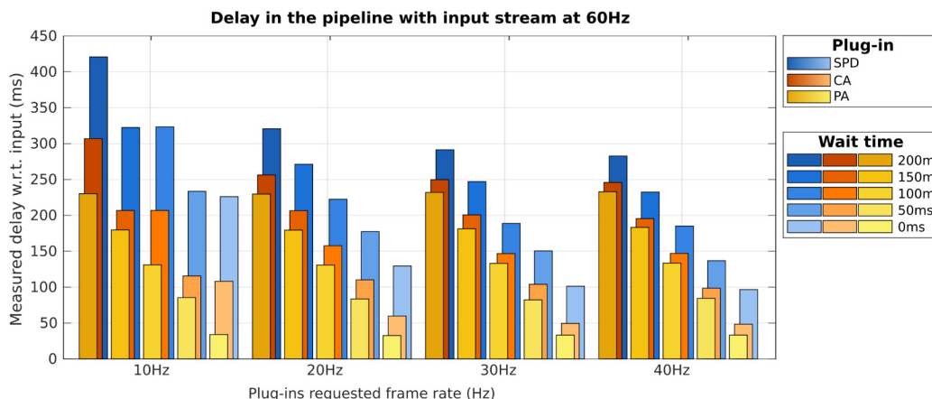
Fig. 3. Measured delay between the output of each plug-in and real-time input stream when plug-ins are connected in sequence: Input \rightarrow Python Algorithm (PA, in yellow) \rightarrow Cpp Algorithm (CA, in orange) \rightarrow SonoNet (SPD, in blue). The increasing wait time introduced in the PA plug-in is coded in the lighter to darker shade for each plug-in. When a higher frame-rate is requested, the delay decreases until around 30 Hz where other system parameters (e.g. memory, CPU, etc.) become the limiting factor. (For interpretation of the references to color in this figure legend, the reader is referred to the web version of this article.)
