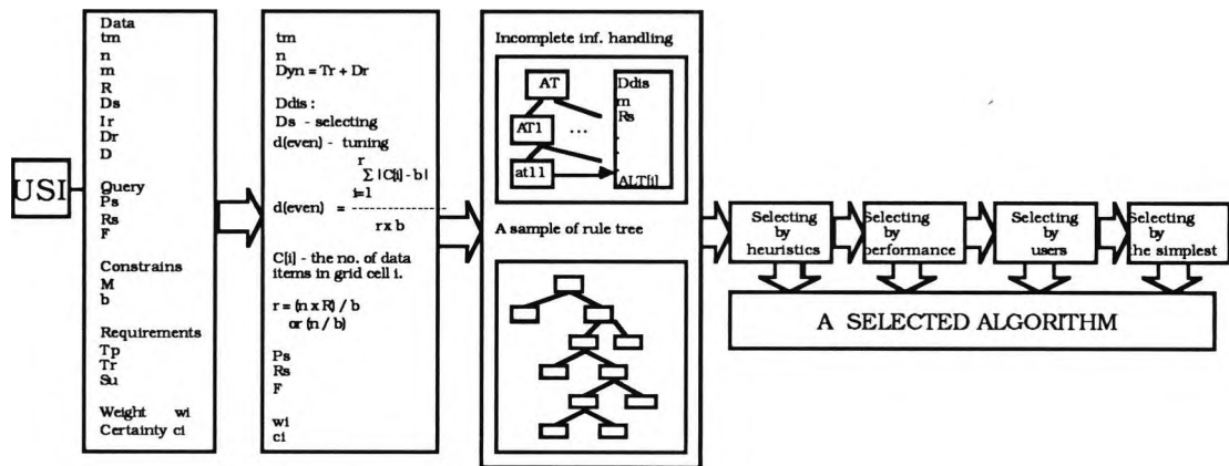
Figure 3.4 A Framework of Initial Algorithm Selection.
