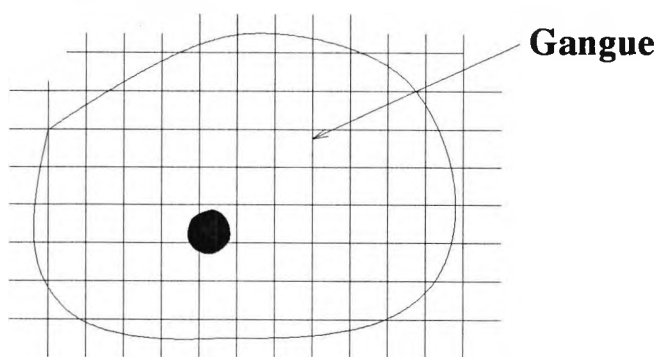
Figure 5.15: Fragment of bulk material with product and gangue.
