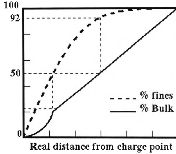
Figure 2.7: Effect on Segregation by Particle Size
