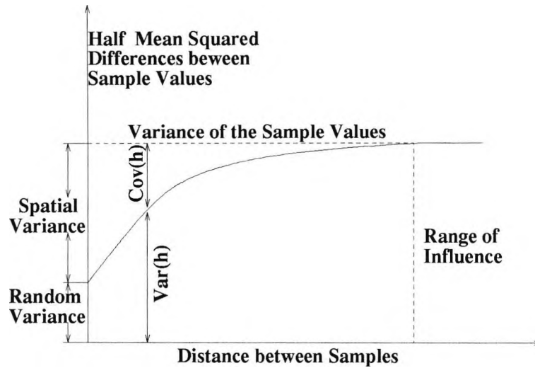
Figure 3.7: A typical Variogram showing relationship among Variance, Covariance and Variogram.
