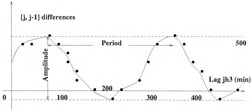
Figure 3.4: Periodic Variogram \gamma_{f3}(\theta) for the simplest f_3(t) considered.
