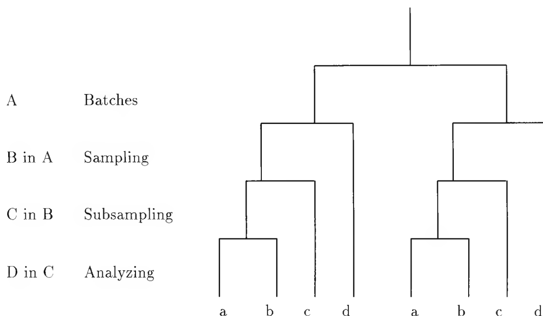
Figure 4.3: Staggered Nested Design.
