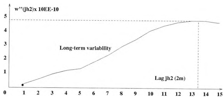
Figure 3.11: Graphical Representation of the Experimental Variogram V(j) of Long-term Charcoal Fluctuations. Quality Characteristic: Particle Size.
