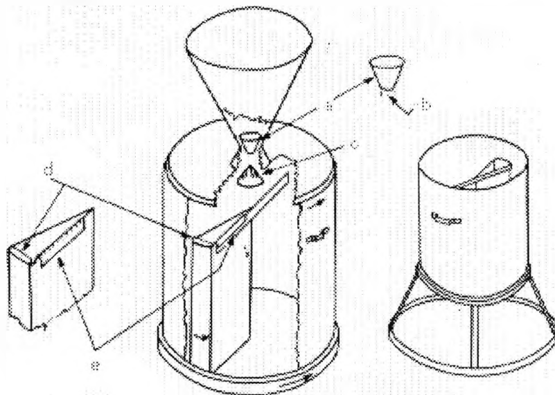
Figure 5.11: Rotary Sampler Divider with Hopper, Cone and Stand.
