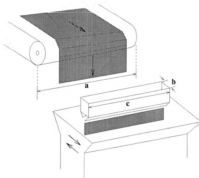
Figure 5.2: Conveyor Belt with Falling-stream Sampler: through-stream, cutter-bucket Type.
