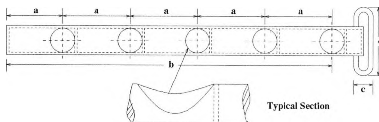
Figure 5.21: Accessories: Tubular Sampling Spear.
