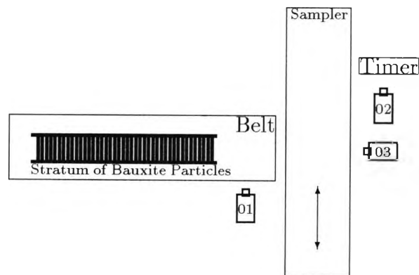
Figure 5.7: Schematic Layout of the Experiment for Critical Design Parameters.
