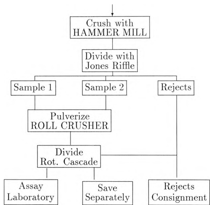
Figure 5.16: Flow sheet for Particle Size Reducing
