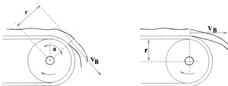
Figure 5.9: Trajectory of Material when leaving the Conveyor Belt with high and low tangential speed, respectively.
