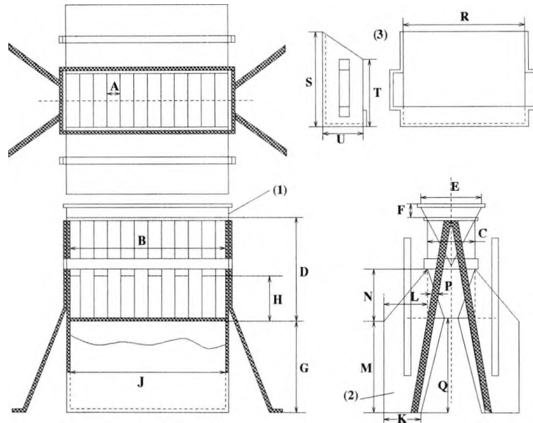
Figure 5.10: Top, Side and Front View for Jones Riffle Design.
