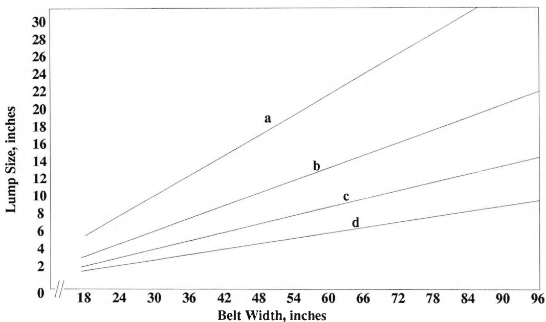
Figure 5.8: Belt width required for a given lump size.
