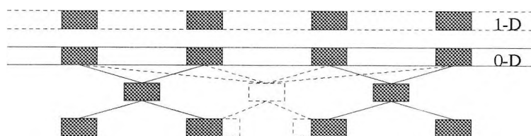
Figure 1.1: Arrangements of increments and replications within the boundaries of specified precision.
