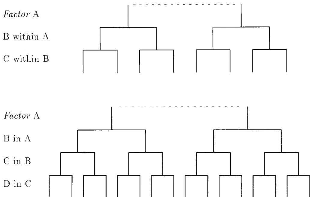
Figure 4.2: Three and Four-Stage Balanced Nested Designs.
