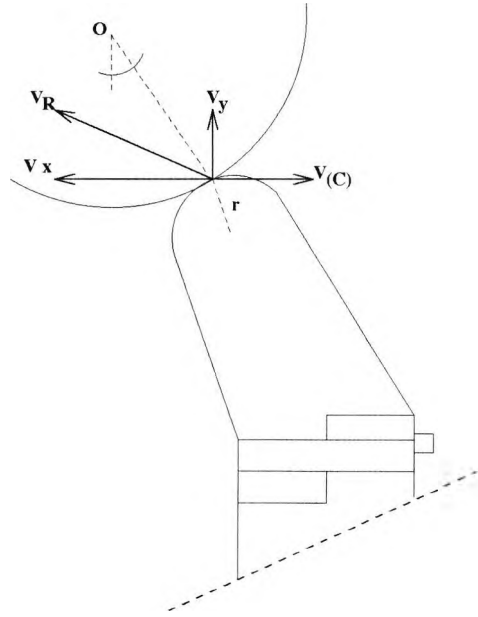
Figure 5.4: Collision of Particle with cutter edge.
