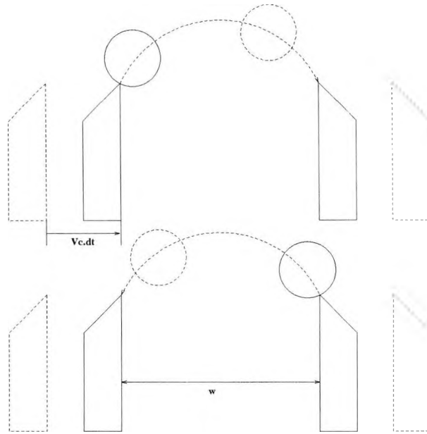
Figure 5.5: Collision of Fragments with Opposite Edges of the Cutter.
