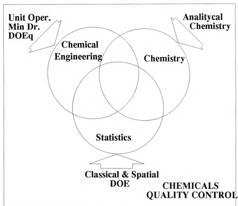
Figure 1.2: Relationship among areas studied in this work.
