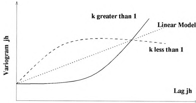
Figure 3.5: Linear and Generalized Linear Model for \gamma_f(\theta) = \gamma_{f1} + \gamma'_{f2}\theta^k .
