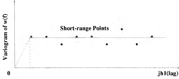
Figure 3.2: Flat Variogram \gamma_{f1}(\theta) for f_1(t) with random distribution.
