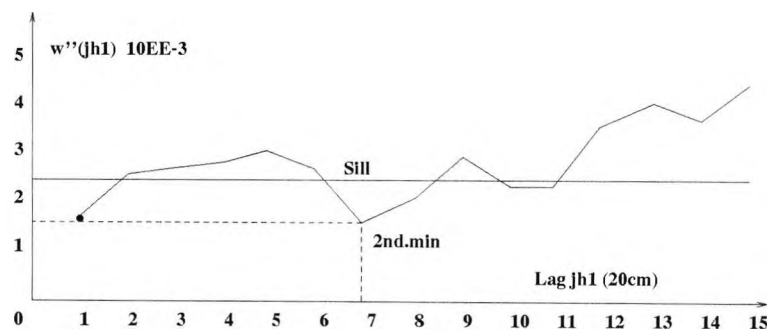
Figure 3.10: Graphical Representation of the Experimental Variogram V(j) of Short-term Charcoal Fluctuations. Quality Characteristic: Particle Size.
