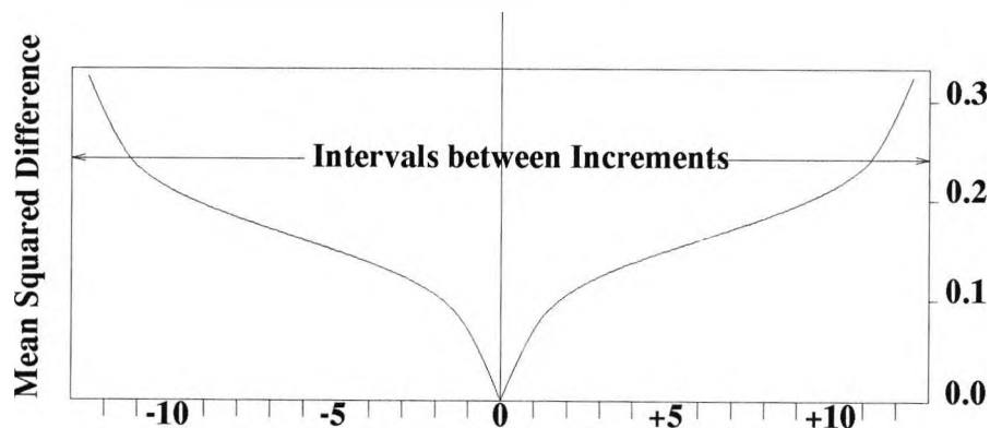
Figure 3.8: The Symmetrical Semivariogram with One-dimensional Variations.
