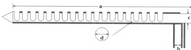
Figure 5.22: Accessories: Shuttered Sampling Spear for Dry, Free running Solids.
