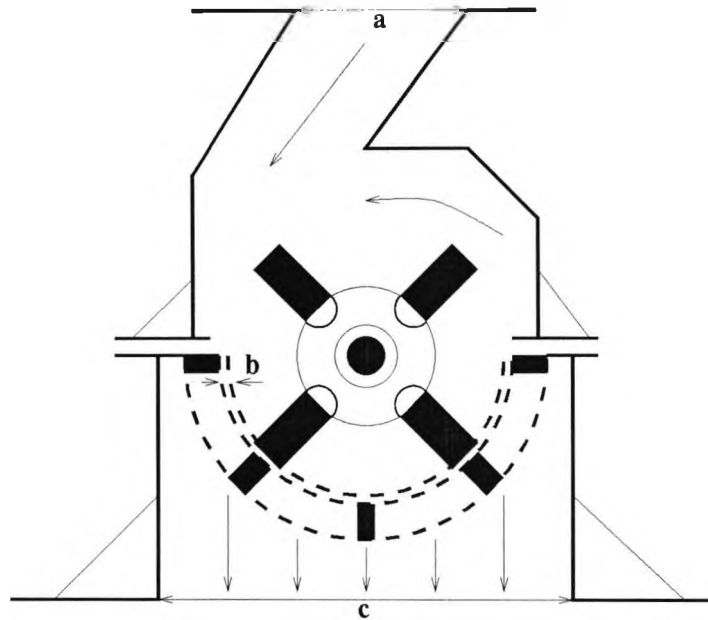
Figure 5.17: Typical Hammer Mill for Pilot Experiments. Courtesy, Pascall Engineering.
