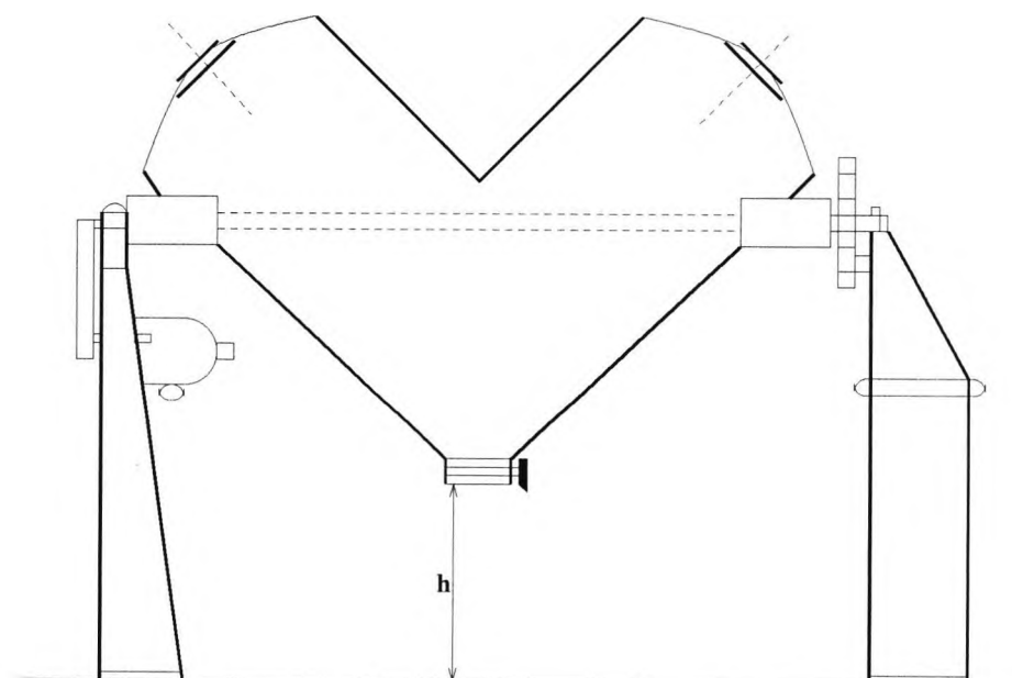
Figure 5.13: Industrial Solids-mixing Machine.
