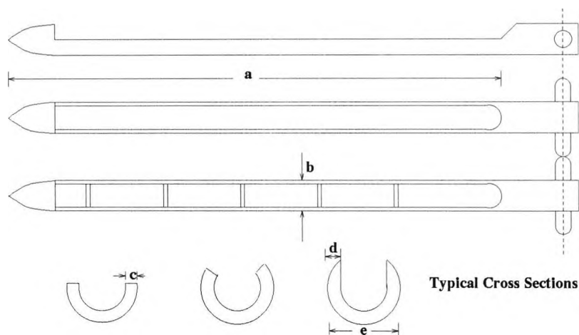
Figure 5.20: Accessories: Open-sided Sampling Spear and Divided Spear for Dry, Free-running Powders.
