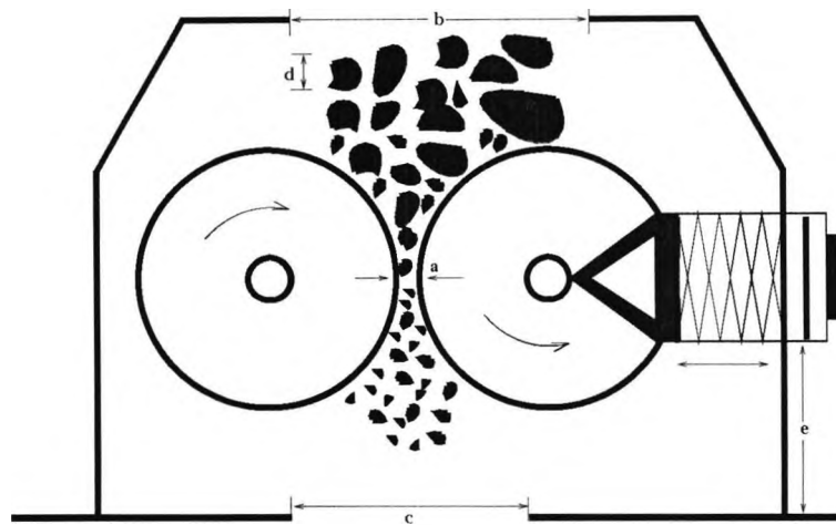
Figure 5.18: Schematic Representation of Double Roll Crusher with Spring-loaded Roller.
