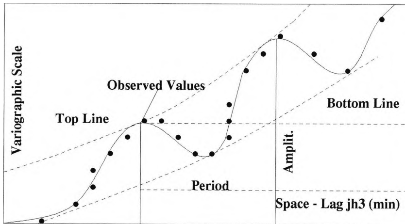
Figure 3.6: Graphical Representation of Periodic Variogram and Method for determination of both Period ( T_P ) and Amplitude ( \gamma_{f3} ).
