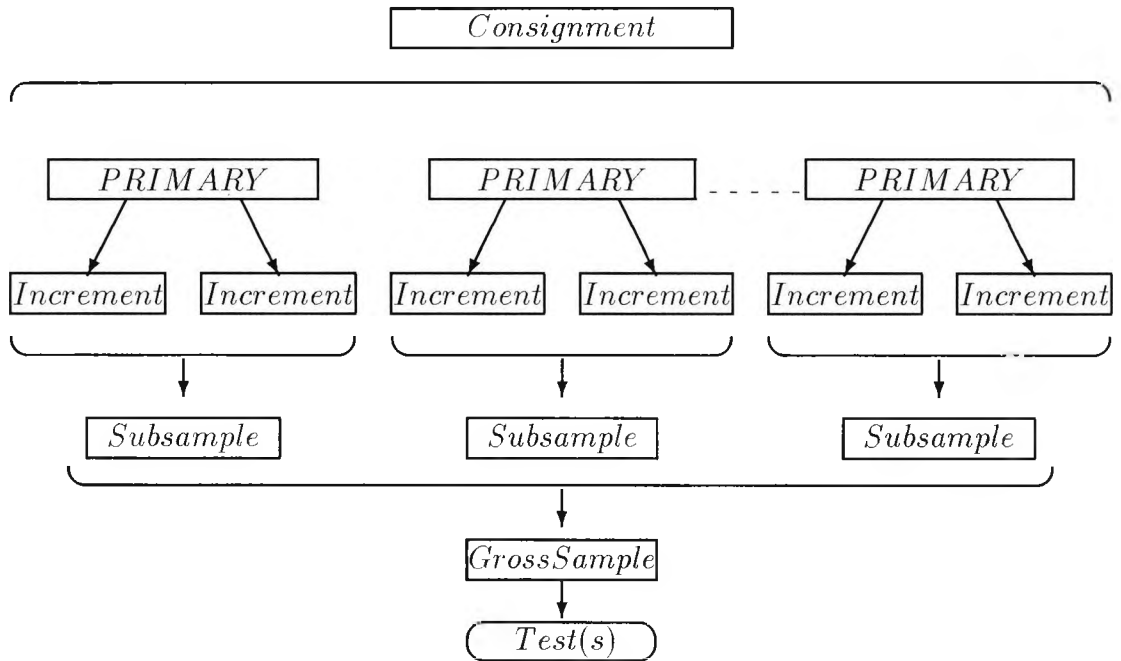
Figure 2.11: Two-stage sampling with primary and secondary sampling units.
