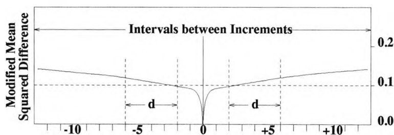
Figure 3.9: The Modified Semivariogram for Computation of Standard Error.
