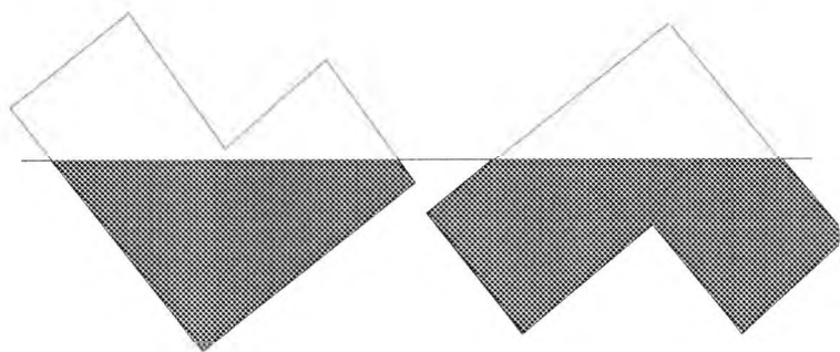
Figure 5.12: Principle of Unequal Displacement.
