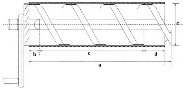
Figure 5.24: Accessories: Shuttered Sampling Auger.
