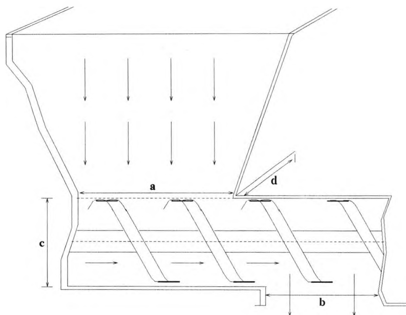
Figure 5.19: Typical Screw Feeder for Sampling Station.
