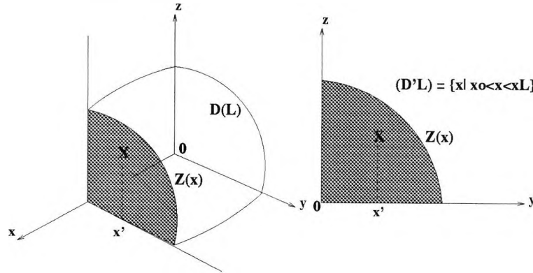
Figure 2.3: Slice of an elongate Pile considered three-dimensional but represented by a one-dimensional model over the x axis.
