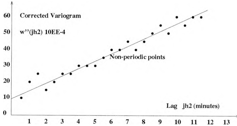
Figure 3.3: Long-range continuous Variogram \gamma_{f2}(\theta) for f_2(t) with autocorrelation.
