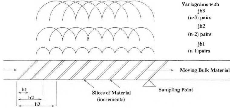
Figure 3.1: Schematization of Terms to Compute a Variogram, where h1 = \theta , h2 = 2\theta and so on, r = h/\theta and n = T/\theta .
