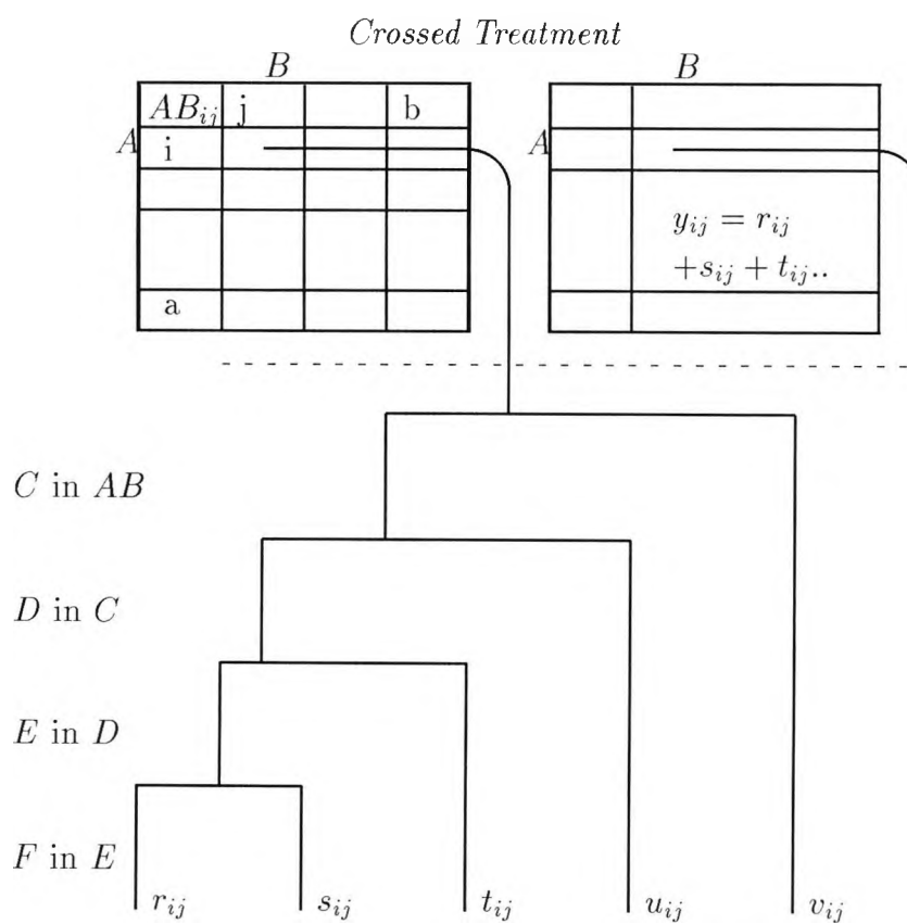
Figure 4.4: Balanced Nested Factorial Design.
