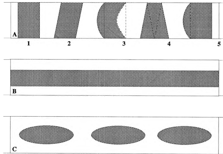
Figure 5.3: Taking increments: Correct Delimitation only with parallel cuts across the stream.
