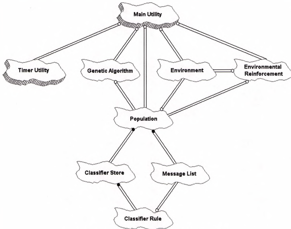
Class Diagram of the Classifier System
