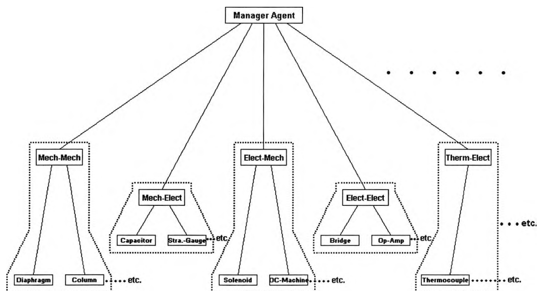
Figure 3.2 The Control Structure of the DPS system
