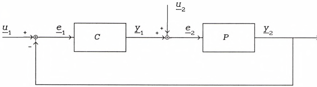
Figure (8.1): The MIMO unity feedback configuration
