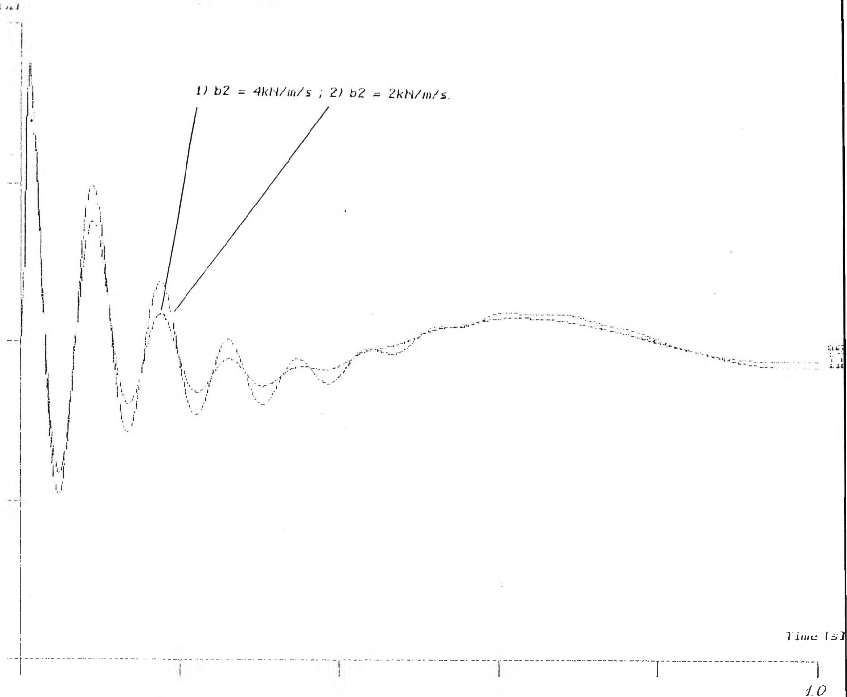
Fig. 5.6 Effect of Suspension Damping b_2 on z(t) at v = 80 \text{ km/h} h = 0.01 \text{ m}
