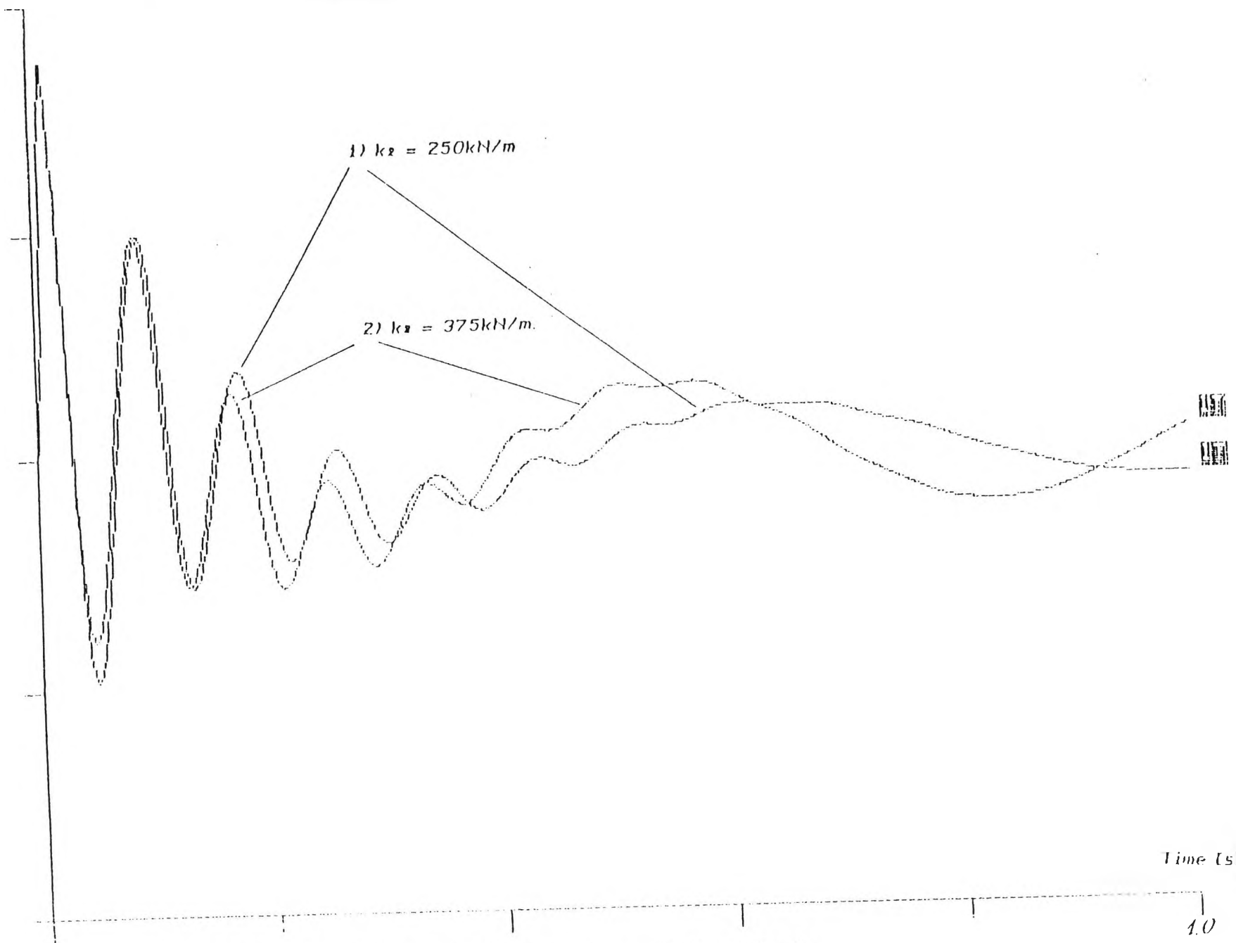
Fig. 5.5 Effect of Suspension Stiffness - k_2 on IF: U = 80 \text{ km/h} ;
