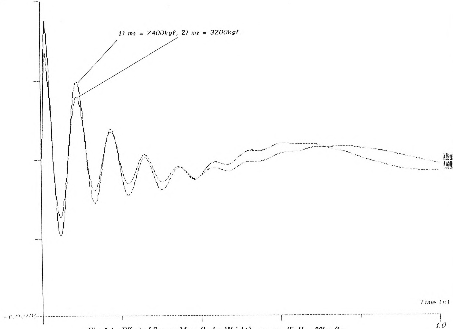
Fig. 5.4 Effect of Sprung Mass (Laden Weight) - m_2 on IF: U = 80\text{km/h} ; h = 0.01\text{m} ; 1) m_2 = 2400\text{kgf} , 2) m_2 = 3200\text{kgf} .
