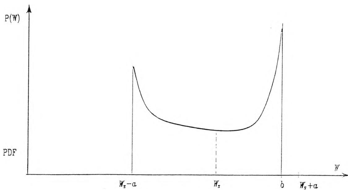
(b) PDF for a Non-linear suspension signal
