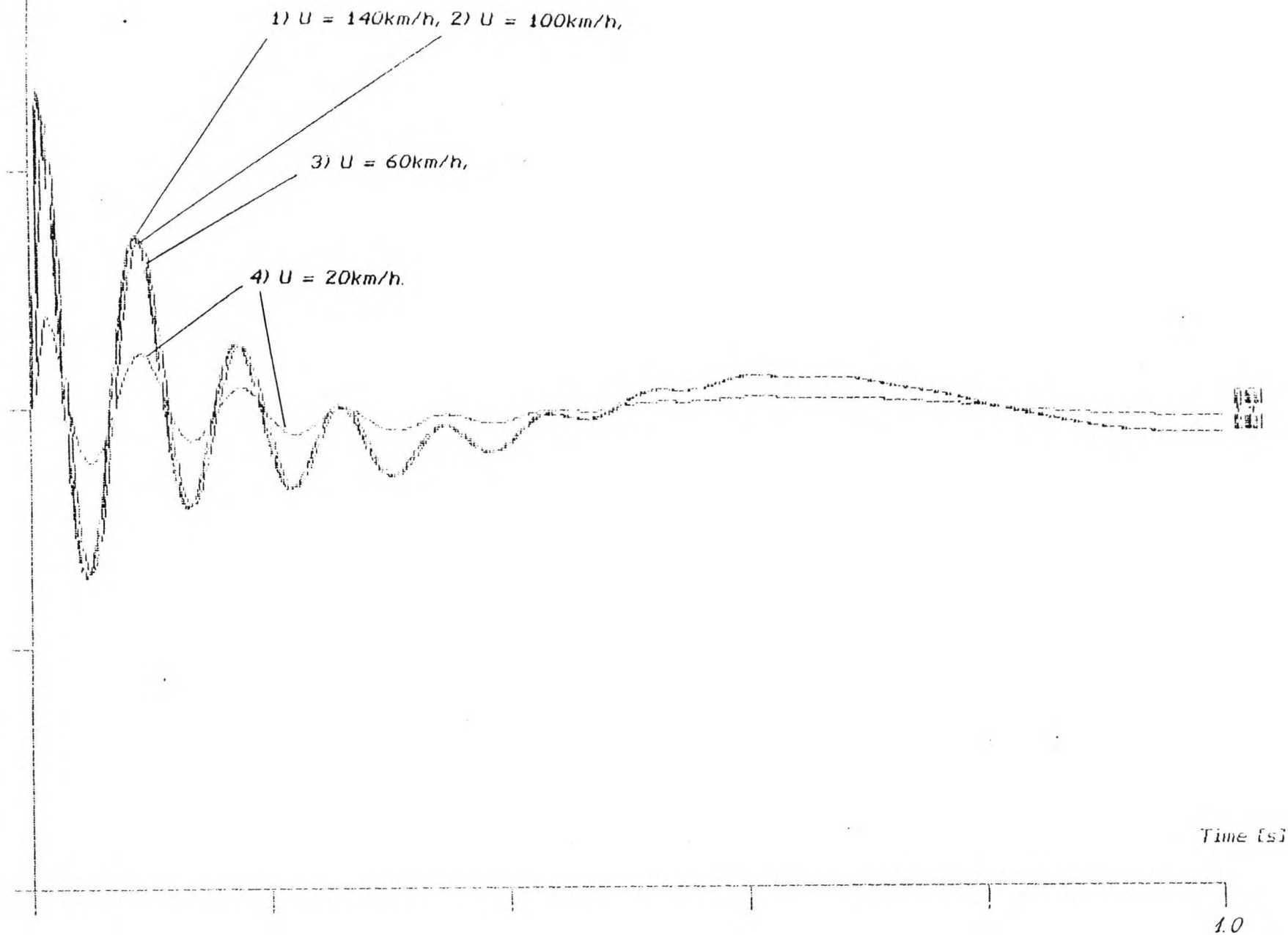
Fig. 5.2 Effect of Vehicle horizontal Speed - U on IF : h = 0.01 \text{ m} ;
