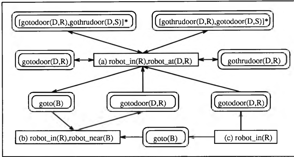
Figure 5.2: G'_{robot} after loop updating
