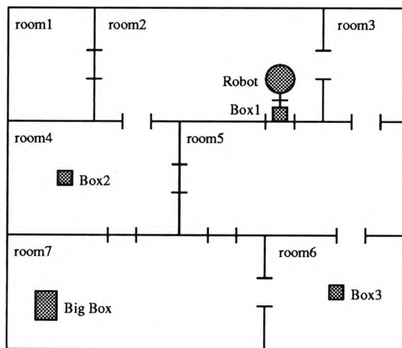
Figure 3.1: Example Problem SW
