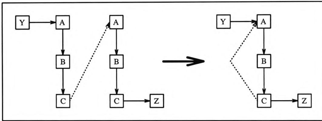
Figure 8.1: Formation of Iterative Macros
