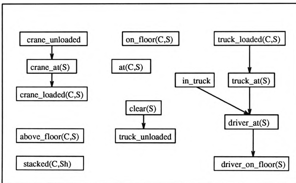
Figure 4.8: WW: PRECEDE goal order
