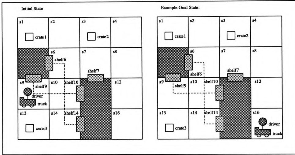
Figure 6.1: WW: example problem
