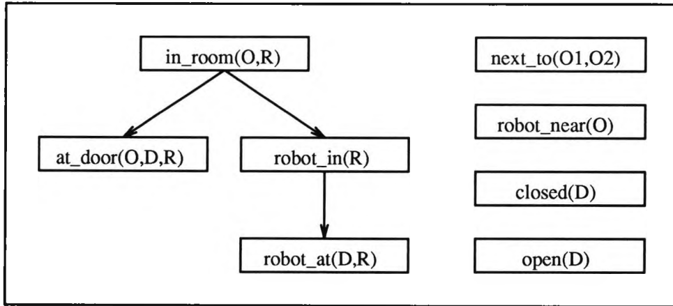
Figure 4.5: SW : PRECEDE partial order
