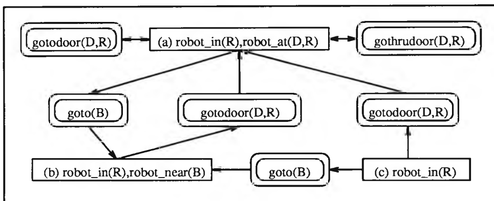
Figure 5.1: G_{robot} : sample output from propose_graphs
