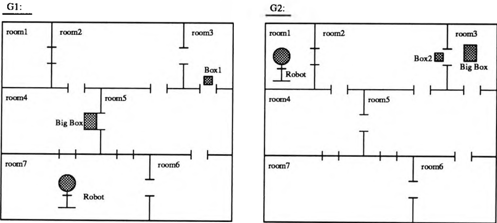
Figure 4.7: Example SW Planning Goals
