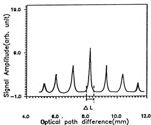
Figure C.3 Illustration of semi-visibility function (a.c. component) of a multimode laser diode.
