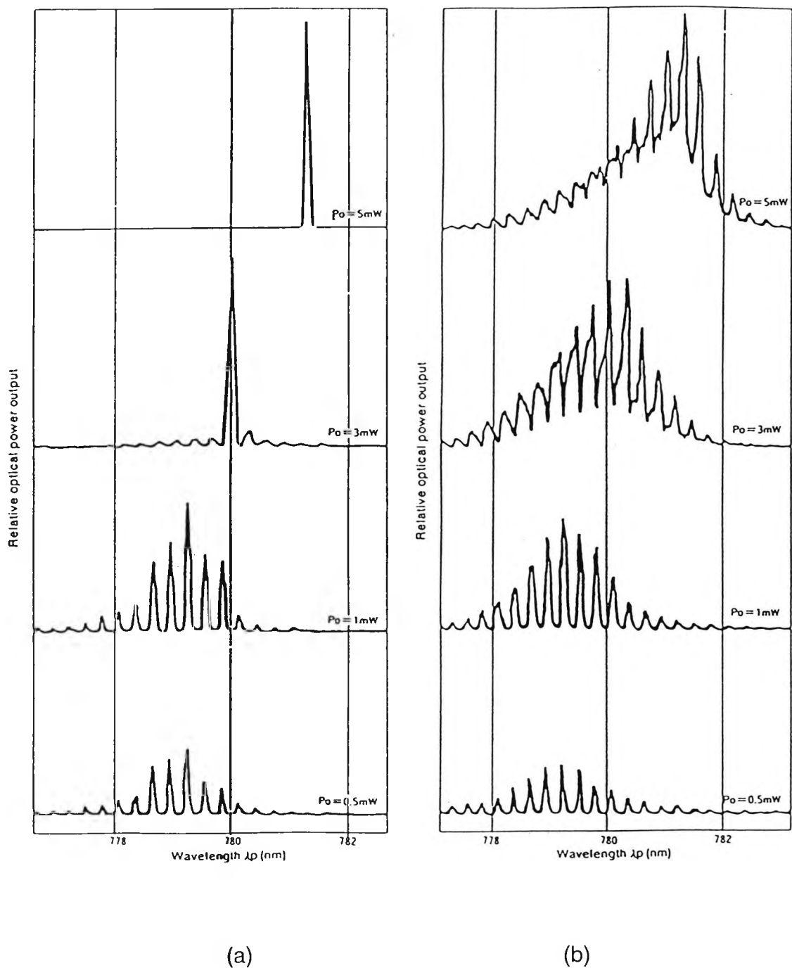
Figure 1.5 Spectral output characteristic of laser diodes: (a) Single mode, (b) Multimode.
