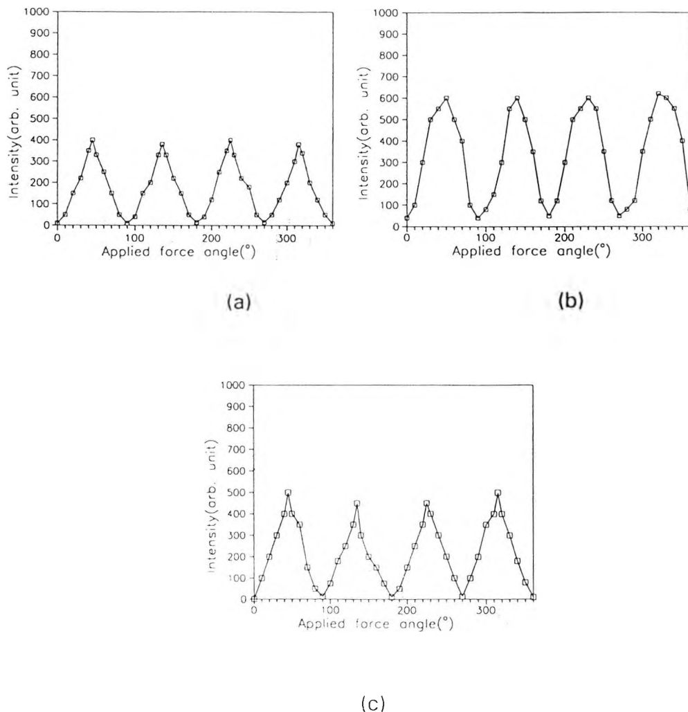
Figure 5.9 Plot of signal amplitude against applied force angle using: (a) Bow-tie, (b) E-series, and (c) D-series fibres.
