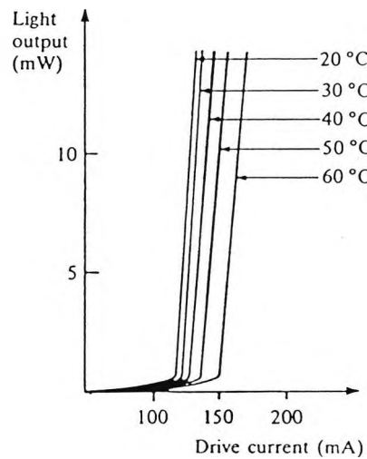
Figure 1.6 Laser diode output power versus drive current for a series of temperatures.
