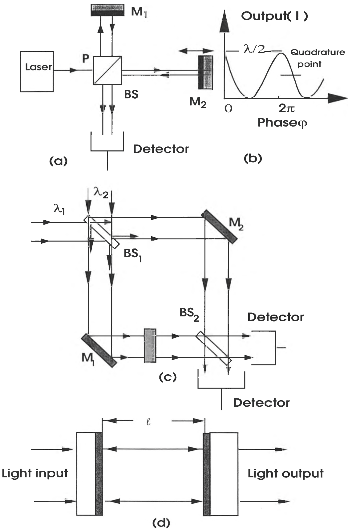
Figure 1.8 (a) Schematic representation of Michelson interferometer, (b) Plot of the Michelson interferometer output intensity as a function of phase \phi , (c) Mach-Zehnder and (d) Fabry-Perot interferometers.
