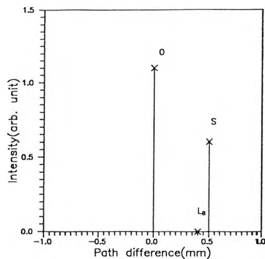
Figure 3.8 Visibility of interference fringes with an applied force, L_B denotes the reference, bias position due to Hi-Bi fibre, S the peak signal position and O the central order.
