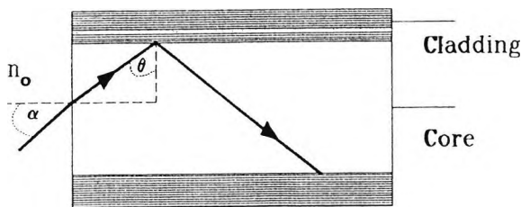
Figure 1.15 Illustration of light coupling into optical fibre.
