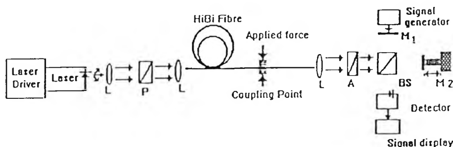
Figure 5.5 Illustration of the experimental arrangement when one coupling point is applied on the sensing unit: Ls Lenses, P Polariser, A Output polariser, BS Beamsplitter, Ms Mirrors.
