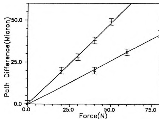
Figure 3.9 Calibration graph showing the changes in path difference of the interference signals against applied force in biased scheme for the Araldite(+) and Perspex(x) samples at a temperature of 20°C.
