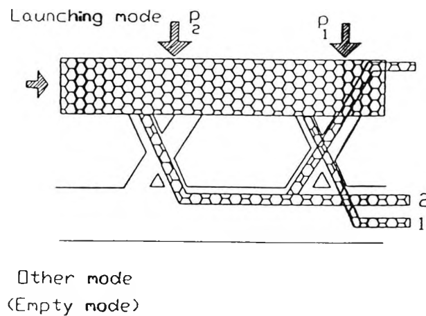
Figure 5.2 Illustration of the mode-coupling of light propagating in a Hi-Bi fibre when 2 coupling points ( p_1 , p_2 ) are applied to it.
