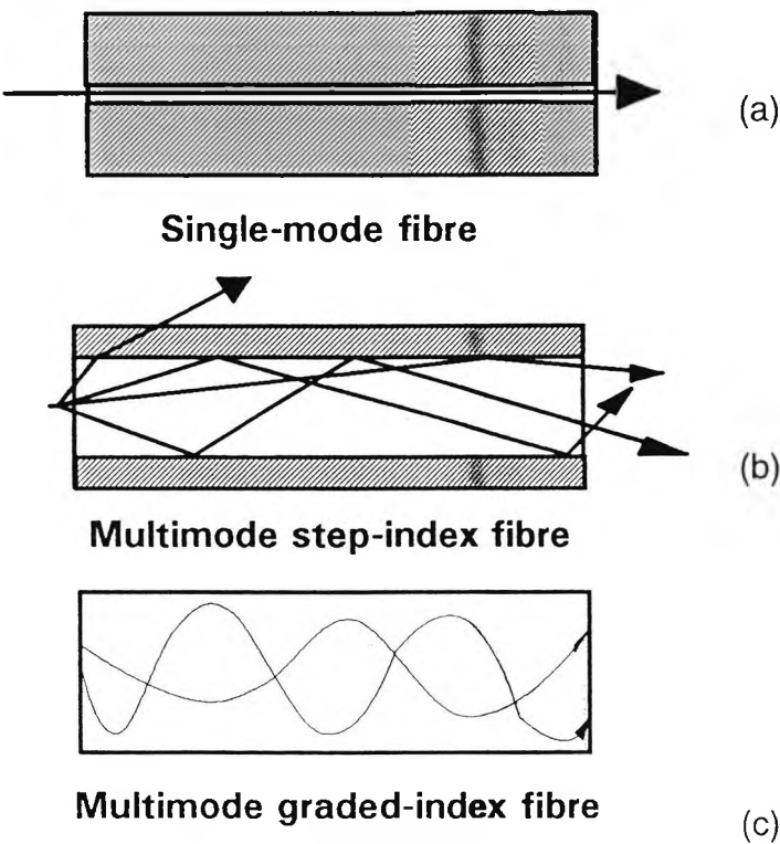
Figure 1.16 Characteristic of light propergation in optical fibres: (a) Single mode fibre, (b) Step-index fibre with multimode propagation, (c) Graded-index fibre with multimode propagation.
