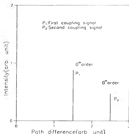
Figure 5.3 Illustration of the 0th order peak of the interferometer output when two coupling points are applied to the fibre, with light launched into one mode of a Hi-Bi fibre and with the polariser crossed.
