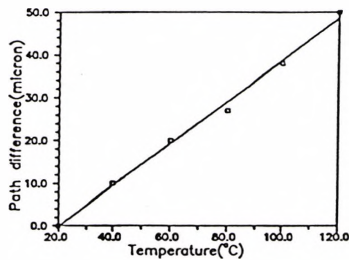
Figure 5.17 Plot of optical path difference against temperature using Bow-tie fibre.
