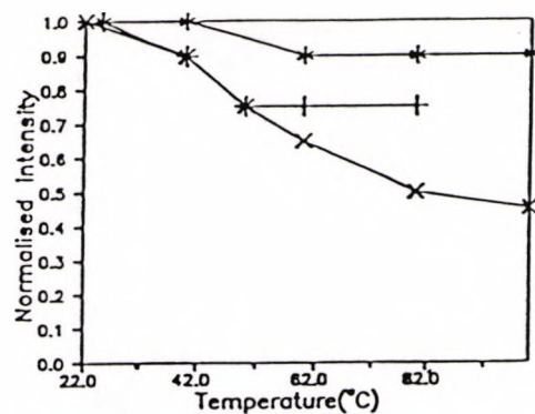
Figure 5.16 Plot of the normalised intensity against temperature using : Bow-tie(x), E-series(*), and D-series(+), for increasing temperature.
