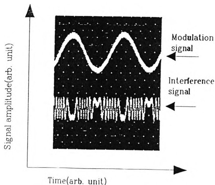
Figure 3.3 Illustration of the signal intensity of the interference signal recorded on the detector in the interferometer, and the modulation source.
