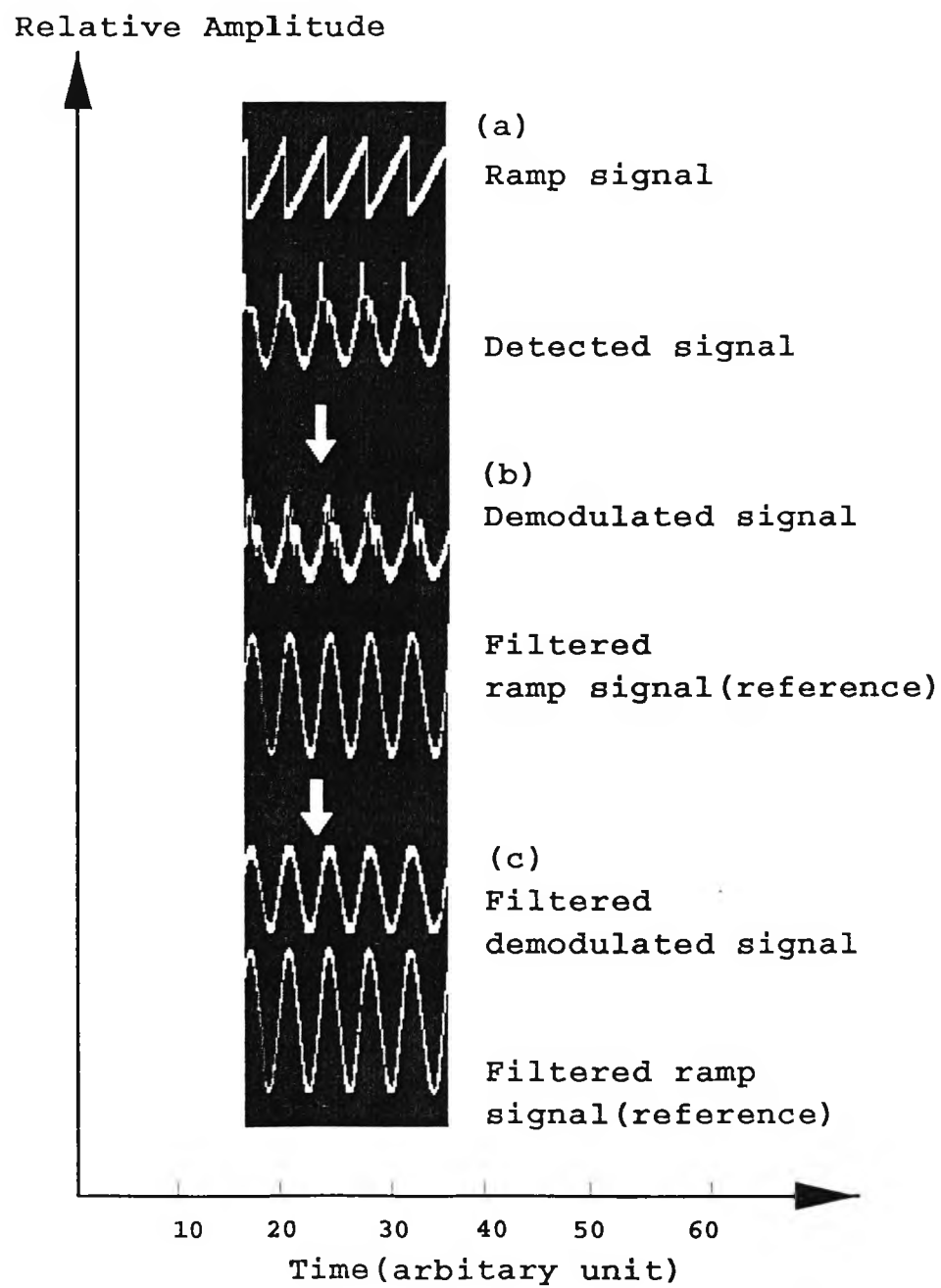
Figure 2.6 Illustration of interferometer output signals obtained from oscilloscope.
