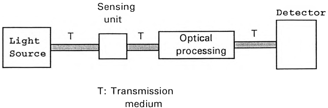
Figure 1.1 Schematic of an optical system arrangement for pressure sensor applications.
