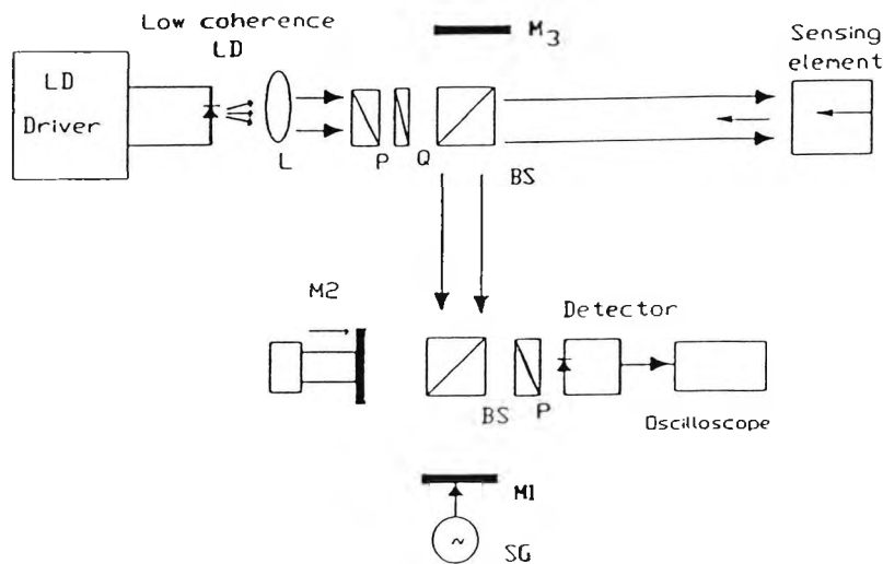
Figure 3.2 Schematic diagram of the experimental arrangement used in reflection: LD Laser diode, Q Half-wave plate, BS Beamsplitter, Ms mirrors, Ls Lenses, SG Signal generator, Ps Polarisers.
