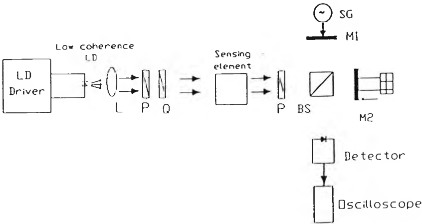
Figure 3.4 Schematic diagram of the experimental arrangement used in transmission : LD Laser diode, Q Half-wave plate, BS Beamsplitter, Ms mirrors, Ls Lenses, SG Signal generator, Ps Polarisers.
