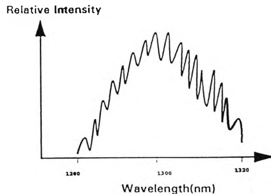
Figure 1.7 Spectral output of a superluminescent diode.
