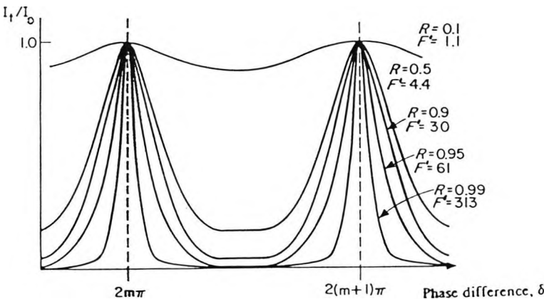
Figure 1.9 Schematic diagram showing the output intensities as a function of mirror reflectance R .
