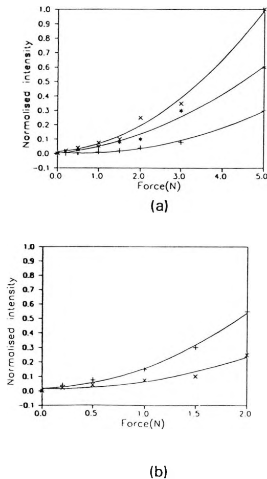
Figure 5.12 Plot of normalised intensity against applied force using D-series fibre: (a) at applied force angle of 0^{\circ} (x), 22.5^{\circ} (*) and 45^{\circ} (+), coupling tooth width of 2.5 mm, (b) at applied force angle of 45^{\circ} , coupling tooth widths of 2.5 mm(x) and 0.5mm (+).
