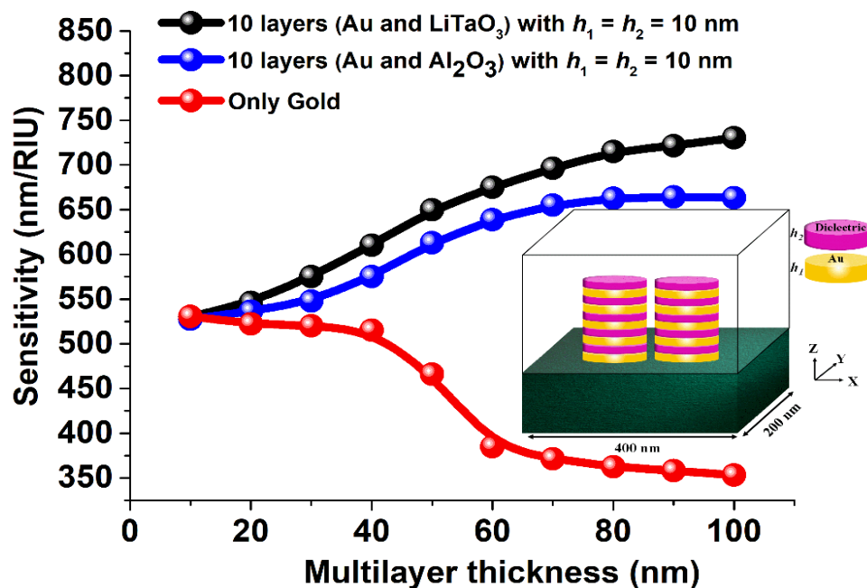
Figure 3. The sensitivity performance of a single metallic (Au) and Al 2 O 3 and LiTaO 3 stacked antenna array when total height, h = 100 nm with or without stacking.
