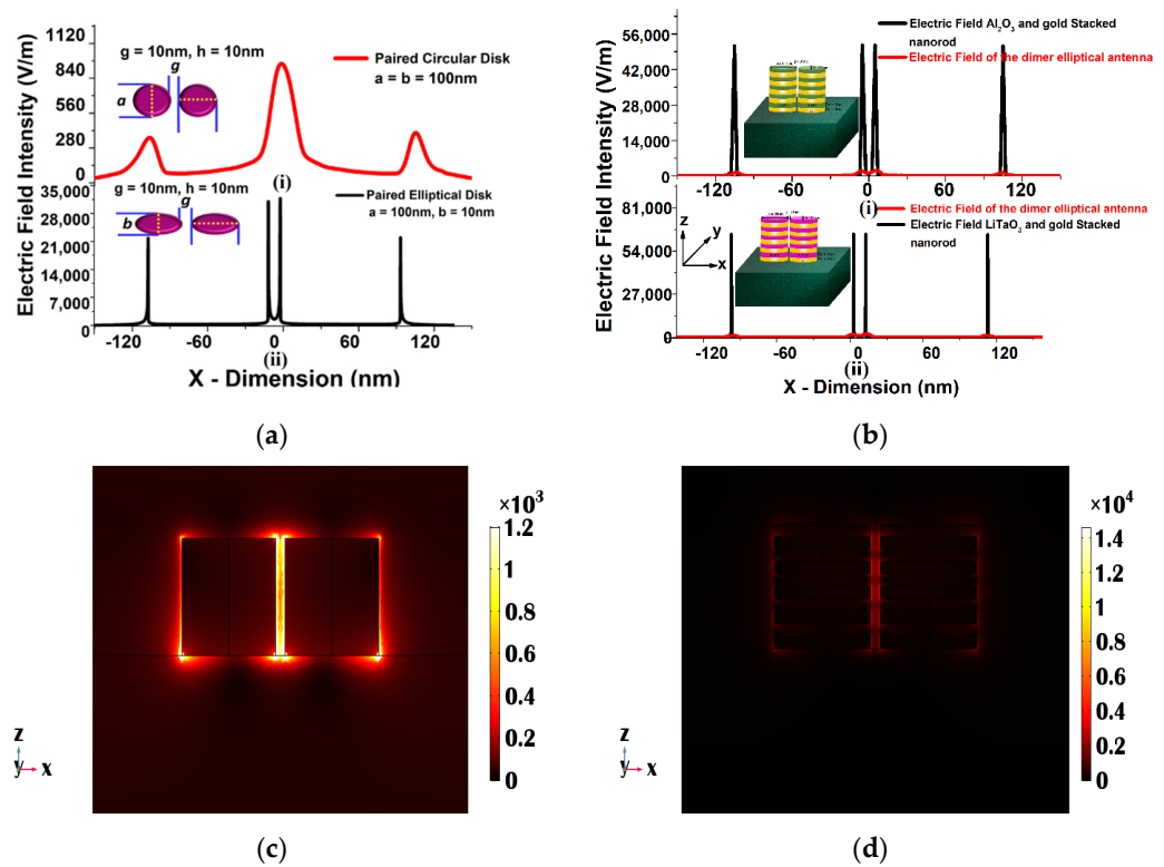
Figure 4. (a) Electric field distribution along the x plane in the gold elliptical and circular paired structure when a = 100 nm, b = 10 , g = 10 nm and h = 10 (b) Electric field distribution along the x plane in the single gold and stacked 10 layers (with \text{LiTaO}_3 or \text{Al}_2\text{O}_3 ) elliptical paired structure when a = 100 nm, b = 10 , g = 10 nm and h_1 = h_2 = 10 nm. (c) E_y , mode field profile at 940 nm wavelength of a single metallic elliptical nano structure when a = 100 nm, b = 10 nm, and h = 100 nm along the x - z plane (d) Electric field variation at 1000 nm wavelength along the x - z plane for a 10 layered \text{LiTaO}_3 stacked nano structure when a = 100 nm, b = 10 nm, and h_1 = h_2 = 10 nm.
