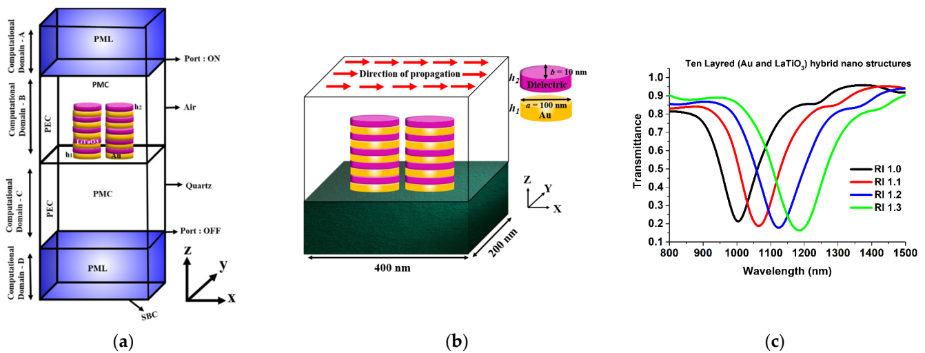
Figure 1. (a) Schematic of the computational domain designed on the FEM method enabled commercial software (b) Graphical representation of the designed hybrid refractive index sensor (c) Transmission spectra of the optimized paired elliptical nano structure with major axis, a = 100 nm and minor axis, b = 10 nm.
