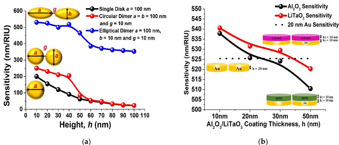
Figure 2. (a) The performance of the single, coupled circular and coupled elliptical shaped gold nano antenna array [66] (b) The sensitivity performance of the two-layer hybrid nanoantenna array.
