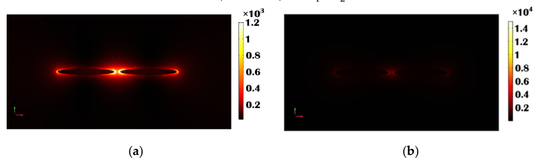
Figure 5. (a) E_x , mode field profile at 940 nm wavelength in the x - y plane of a single metallic elliptical nano structure when a = 100 nm, b = 10 nm, and h = 100 nm, where a slice of the horizontal plane is placed at z = 100 nm. (b) The electric field profile at the 1000 nm wavelength in the x - y plane for a 10 layered \text{LiTaO}_3 stacked nano structure when a = 100 nm, b = 10 nm, and h_1 = h_2 = 10 nm, where the slice of the horizontal plane is adjusted at z = 100 nm.
