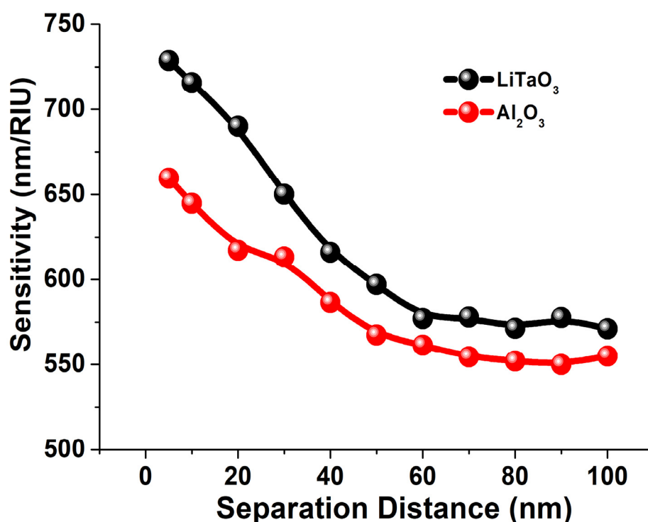
Figure 6. Sensitivity comparison of 10 layered stacked antenna array (5 gold layers with h_1 = 10 nm gold and 5 LiTaO 3 /Al 2 O 3 layers with a = 100 nm, b = 10 nm and h_2 (LiTaO 3 and Al 2 O 3 ) = 10 nm) with respect to separation distance.
