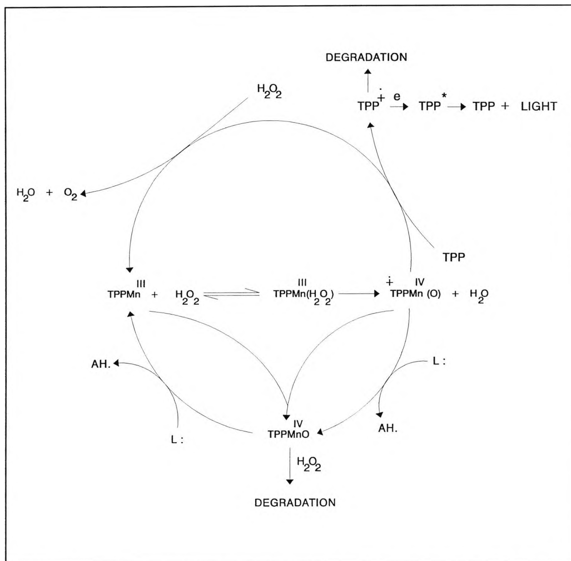
Scheme 8.2 - A summary of the reactions involved in \text{Mn}(\text{T}_{\text{NH}_2}\text{PP})\text{Cl} -catalysed oxidation of luminol by hydrogen peroxide.
