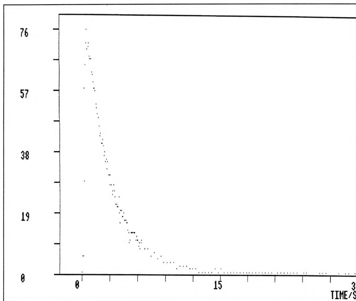
Figure 3.7- Time profile of chemiluminescence from \text{Mn}(\text{T}_{\text{NH}_2}\text{PP})\text{Cl} as oxidised by hydrogen peroxide/ \text{NaOH}(\text{aq.}) .
