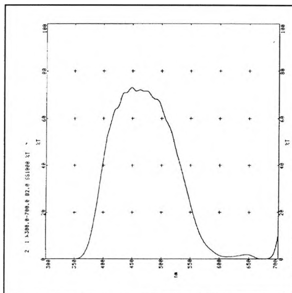
Figure 3.12 - Transmission spectrum of Light Blue filter.
