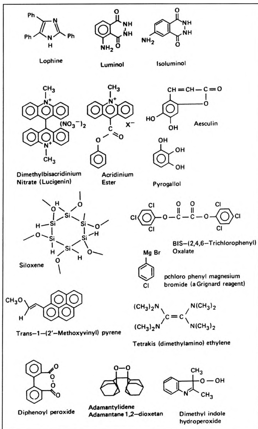
Figure 1.2 - A range of chemiluminescent compounds.
