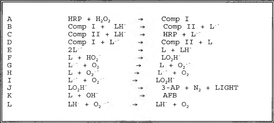
Fig 1.4 - Reactions in the HRP-luminol- \text{H}_2\text{O}_2 system.
