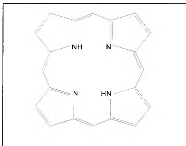
Fig. 1.5 - Porphin
