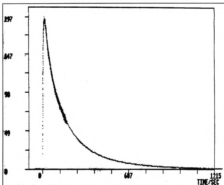
Figure 4.2 - Time profile of chemiluminescence from luminol, as oxidised by \text{H}_2\text{O}_2 and catalysed by \text{Mn}(\text{T}_{\text{NH}_2}\text{PP})\text{Cl} .
