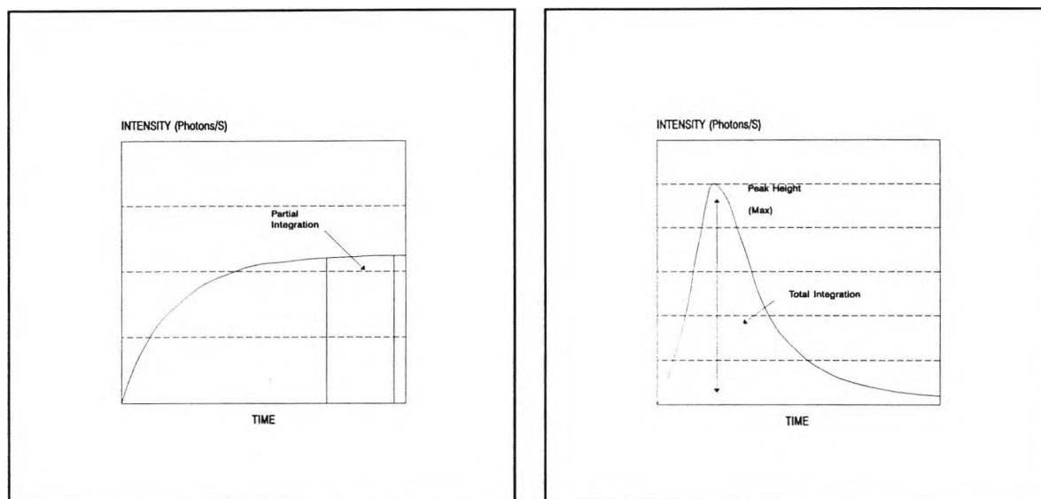
Fig 1.3 - Chemiluminescent reaction profiles
