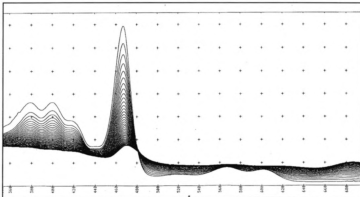
Figure 3.2 - Changes in absorption spectra of Mn(TPP)CL (solvent DMSO/H 2 O 2 ) against time (5 min scan intervals).
