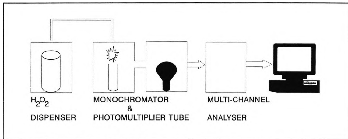
Figure 3.1 - The set up for the measurement of a chemiluminescent spectrum.
