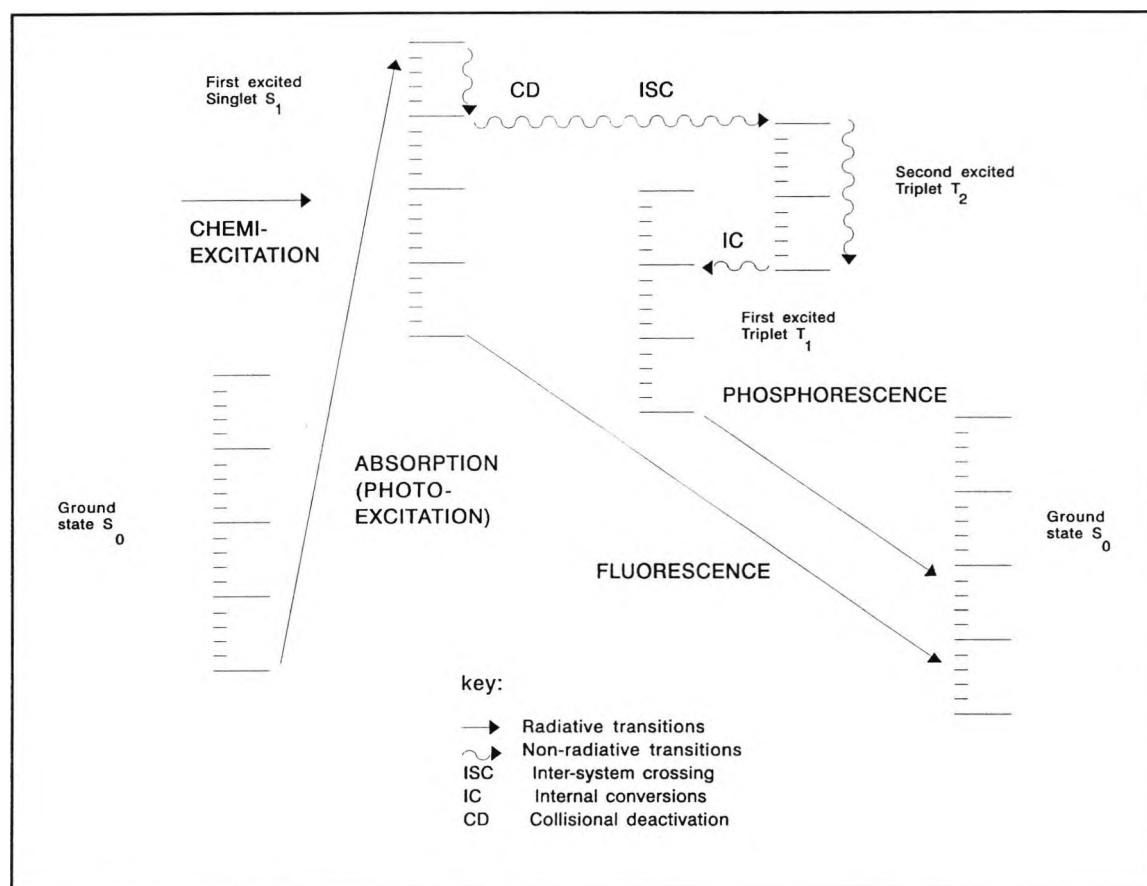
Figure 1.1 - Jablonski diagram
